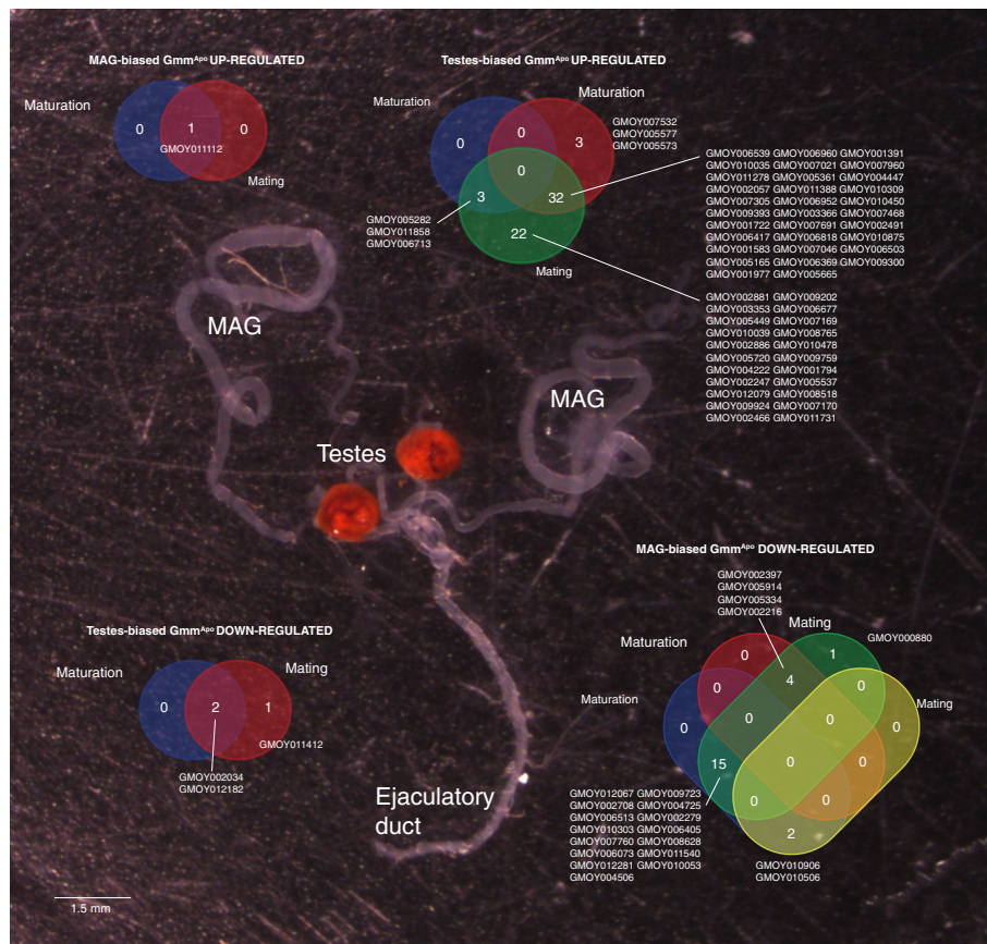
Fig. 4 Genes showing a maturation and mating-responsive transcriptional profile in Gmm^{WT} male reproductive tissues. The IDs of MAGs- and testes-biased genes are shown in Venn diagrams illustrating the number of common sequences found between four groups, i.e. up- or down-regulated in response to maturation and up- or down-regulated in response to mating, separately for MAGs and testes. A tsetse male reproductive tract is shown. Scale bar = 1.5 mm
