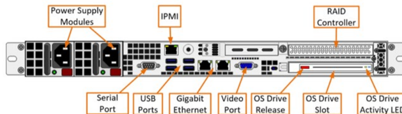
Figure 4. BMC (here labeled IPMI) dedicated management port.
