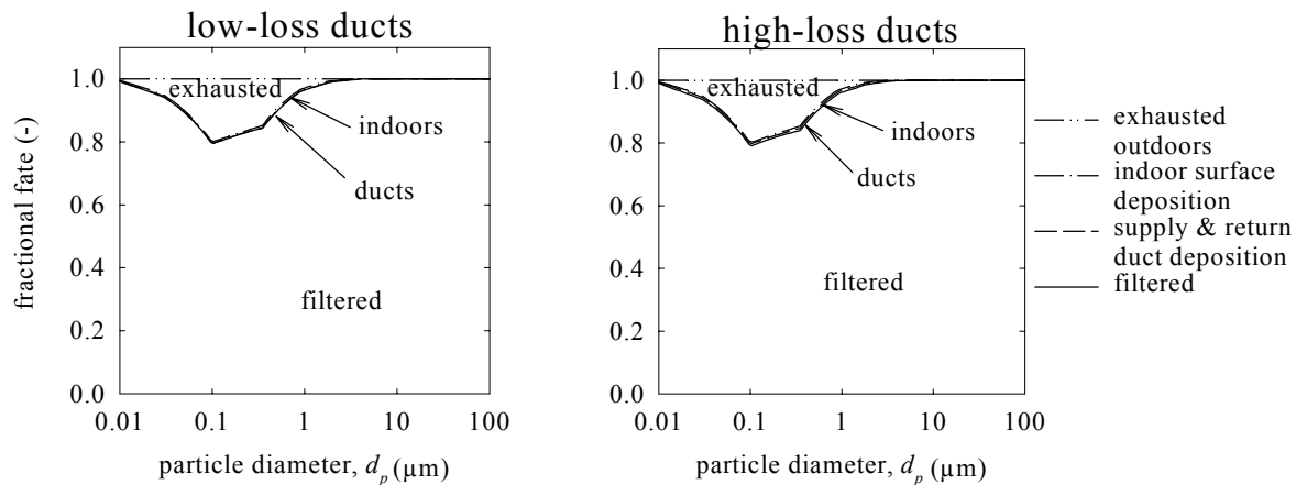
Figure 6 Predicted fractional fates of outdoor particles drawn into an air intake with (a) no filters, (b) 40% ASHRAE filters and (c) 85% ASHRAE filters for both low-loss and high-loss ducts.
