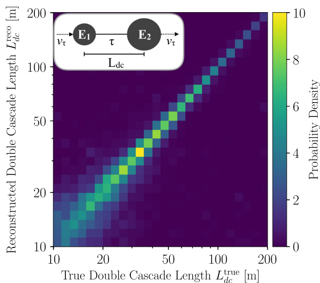
Fig. 1 Length resolution for simulated tau neutrinos classified as double cascades for the best-fit spectrum [19]. With increasing length, the resolution improves while the event expectation drops. The inset shows a schematic of a \nu_\tau CC interaction producing a double cascade with associated reconstruction parameters
