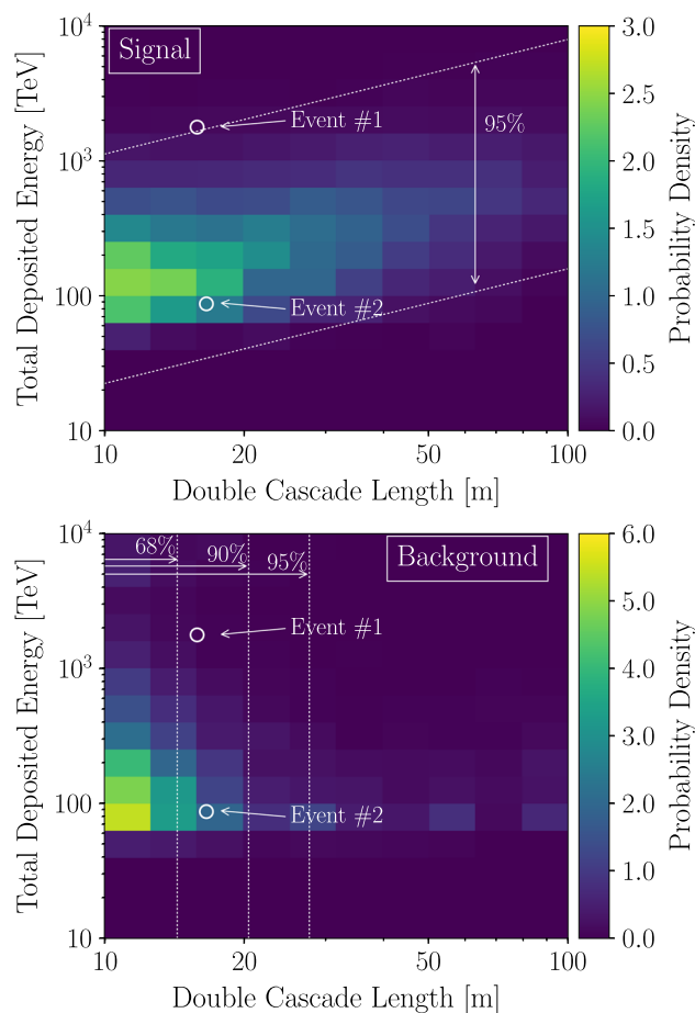
Fig. 2 Two-dimensional MC PDFs showing total reconstructed energy versus reconstructed double-cascade length for the double-cascade subsample with data points, using the best fit to the atmospheric and astrophysical components with the flavor composition of astrophysical neutrinos fixed to 1:1:1 [19]. In the signal ( \nu_\tau -induced double-cascade events) histogram (top), the region containing 95% of the expected signal is indicated with white dotted lines. In the background (all remaining events) histogram (bottom), the white vertical dotted lines mark the regions containing 68%, 90%, and 95% of the single-cascade induced background. In both histograms the two tau neutrino candidates are overlaid as white circles
