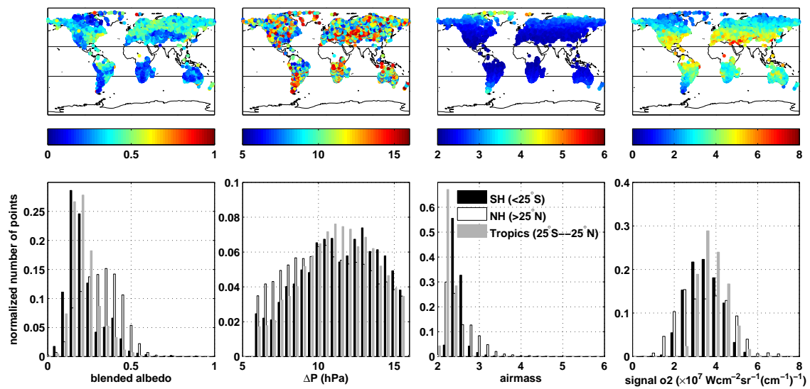
Fig. S1. A map and histogram of the parameters used in equation 4 in August.
