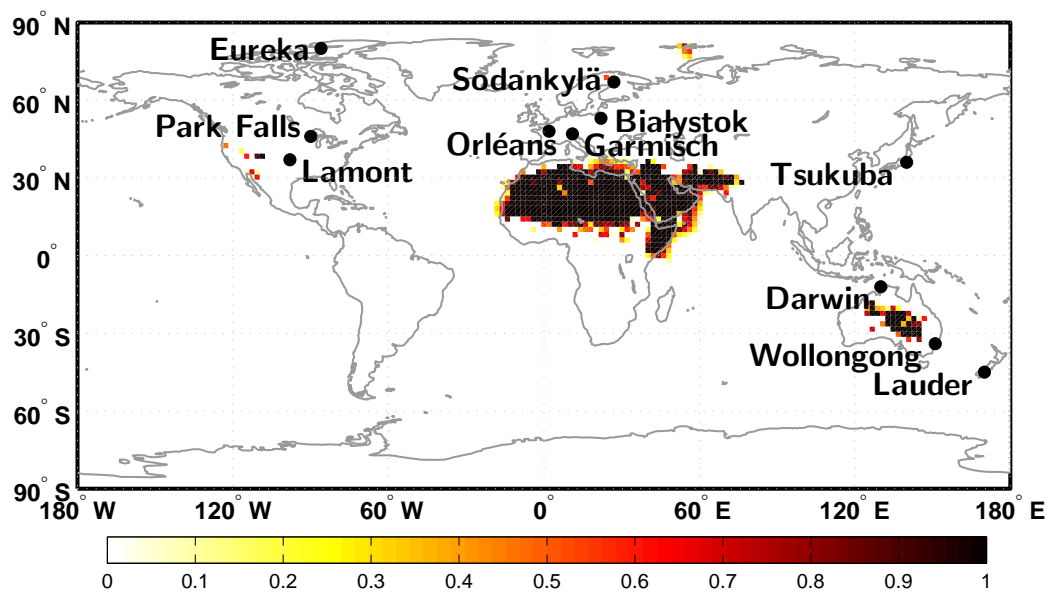
Fig. 1. The locations of the TCCON stations used in this study are shown in black circles. The fraction of soundings in a 2° by 2° box that are M-gain (and removed) are shown in the colours.
