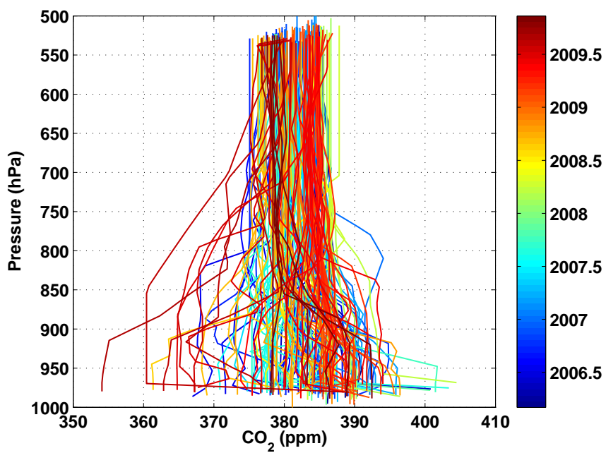
Fig. 7. All the Cessna profiles over Lamont, OK, are shown on a pressure grid, coloured by the time the profile was measured. These profiles are detrended to show only the seasonality and variability.
