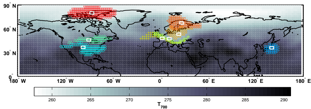
Fig. 11. A map of the areas that fulfill the coincidence criteria for a ten-day period in August, 2010. The background T_{700} field is from the NCEP/NCAR analysis. The white boxes show the \pm 0.5^\circ latitude and \pm 1.5^\circ longitude limits about each TCCON site. The symbols in colour show the locations on the Earth for this ten-day period that satisfy the coincidence criteria that T_{700} is within \pm 2 K, latitude is within \pm 10^\circ , and longitude is within \pm 30^\circ . (The only exception to this is the Tsukuba site, where the longitude criterion is tightened to \pm 10^\circ to avoid over-weighting data over China.) The actual locations of the coincidences with the ACOS-GOSAT data are restricted to the regions overlaid in colour, where the ACOS-GOSAT data exist (i.e., only over land and in cloud-free scenes).
