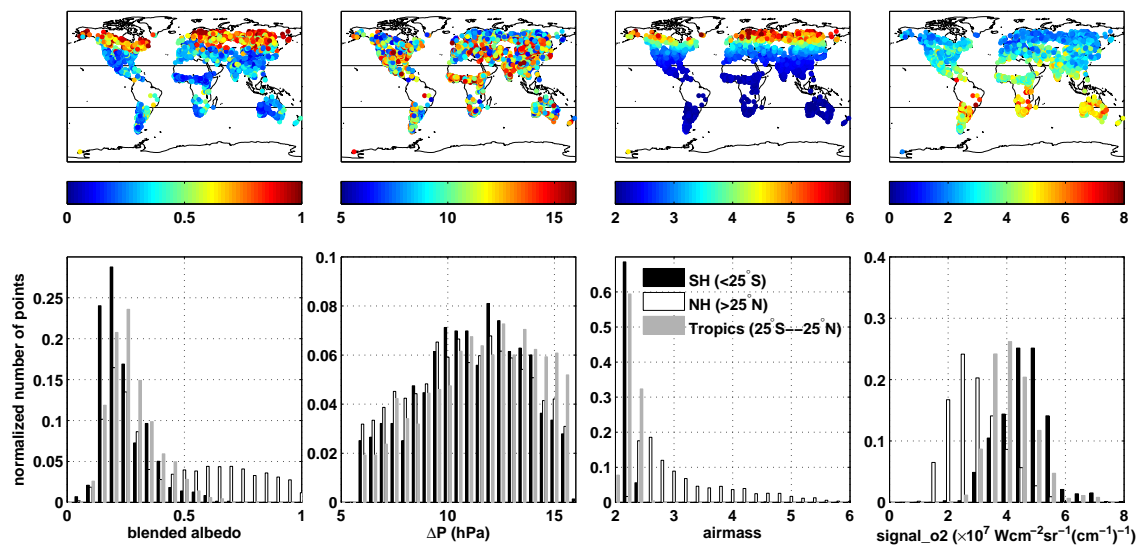
Fig. S2. A map and histogram of the parameters used in equation 4 in February.
