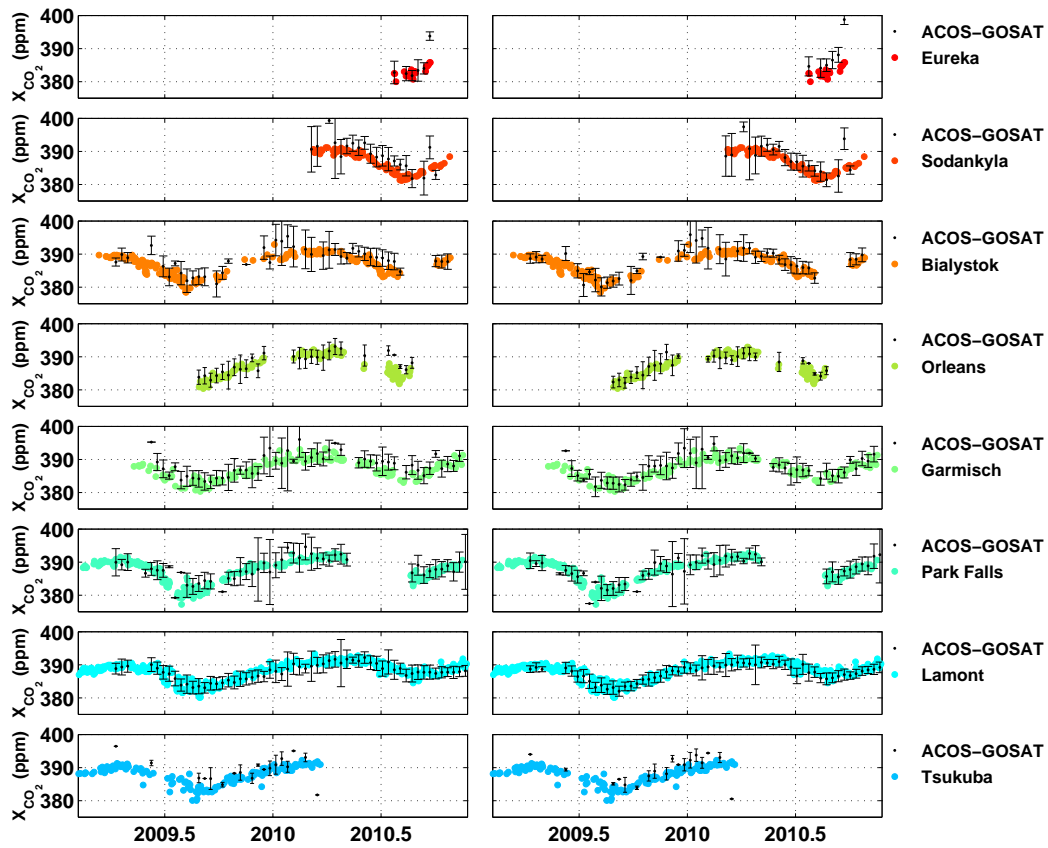
Fig. 12. A site-by-site comparison between ACOS-GOSAT and the Northern Hemisphere TCCON sites, using the T_{700} coincidence criterion (data recorded within 10 days, \pm 10^\circ latitude, \pm 30^\circ longitude and \pm 2K ). The left panel shows the ACOS-GOSAT data after applying the global bias (0.982), and the right panel shows the data after applying Eq. (4).
