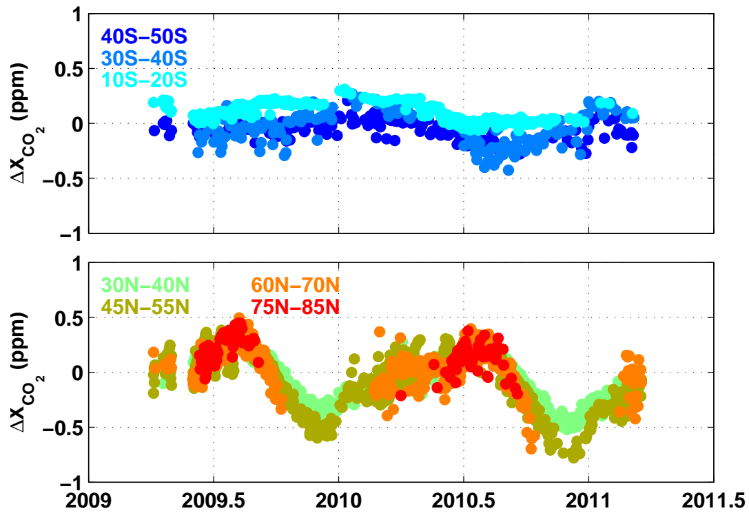
Fig. S3. The latitude-dependence of the difference between using the TCCON a priori profile and the ACOS a priori profile (TCCON–ACOS plotted here) on the ACOS-GOSAT retrievals (e.g., \hat{c}'_1 - \hat{c}_1 from equation A10). The latitudes are binned around TCCON sites.
