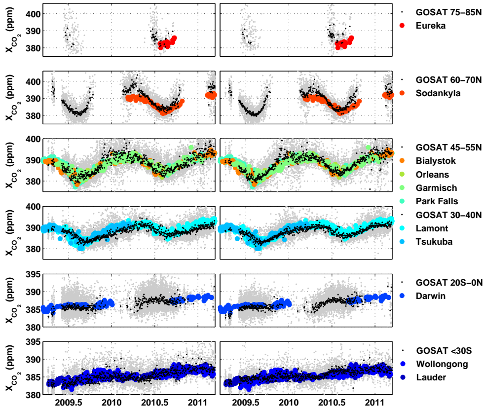
Fig. 9. Seasonal-cycle comparisons. These panels show the ACOS-GOSAT data adjusted by only the global bias (0.982, left panels) and after applying Eq. (4) (right panels). Each row of panels shows a different latitude range for the ACOS-GOSAT data (the black dots are the daily median zonal average values, and the grey dots are the individual measurements), and the TCCON daily median data within the latitude band (multi-coloured circles). The agreement and variability in the ACOS-GOSAT data are visibly improved in the right-hand panels.
