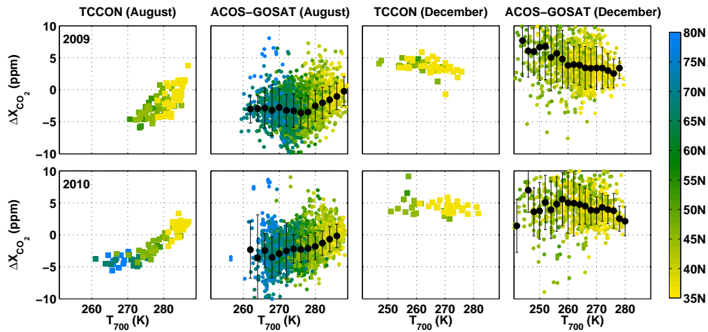
Fig. 10. Plotted here are X_{\text{CO}_2} anomalies against the temperature at 700 hPa. The anomalies are computed by subtracting a 1.89 \text{ ppm yr}^{-1} secular increase from the X_{\text{CO}_2} time series. There is a strong positive relationship in the summertime, and this relationship reverses in sign in the winter. The top row of panels shows data from 2009, and the bottom row shows data from 2010. The first two columns of panels contain data from August, and the right two columns show December. The TCCON data are plotted in squares; the modified ACOS-GOSAT data are circles, and the medians and standard deviations of the ACOS-GOSAT data at each 2 K bin are plotted in black circles with error bars. The colours represent the latitude. Although there are no TCCON data at the highest latitudes (lowest T_{700} ) in 2009, the TCCON sites operating in both years show visibly different drawdown characteristics (indicated by the larger variability in \Delta X_{\text{CO}_2} near 280K) in the August 2009 than in the 2010 TCCON data. This is indistinguishable within the standard deviation of the ACOS-GOSAT data. The ACOS-GOSAT data nicely capture the reversal in sign of the X_{\text{CO}_2} - T_{700} slope in the winter.
