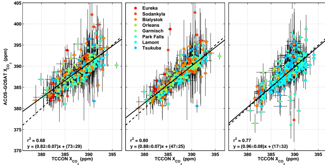
Fig. 13. The left two panels show the regression between TCCON and ACOS-GOSAT using the T_{700} coincidence criterion (10 days, \pm 10^\circ latitude, \pm 30^\circ longitude and \pm 2\text{K} ). The left panel shows the large-scale bias-corrected, but otherwise unmodified, data. The middle panel shows the regression after applying Eq. (4). The right-hand panel shows the regression after applying Eq. (4), but using coincidence criteria that restricts latitudes to within \pm 0.5^\circ , longitudes to within \pm 1.5^\circ , and interpolates the TCCON data onto the ACOS-GOSAT measurement times. Note that there are no coincident data over Eureka when using the geographic coincidence criteria (right-hand panel). The solid lines show the best fit to the data (with equations and \pm 2 standard errors shown on the plot), and the one-to-one line is plotted as a dashed line. The vertical bars represent the \pm 2\sigma variability of the ACOS-GOSAT data, illustrating the dependence of the variability of the ACOS-GOSAT data at each TCCON value (i.e., \text{var}(y|x) ) in the regression. Similarly, the horizontal bars represent the \pm 2\sigma variability of the TCCON data.
