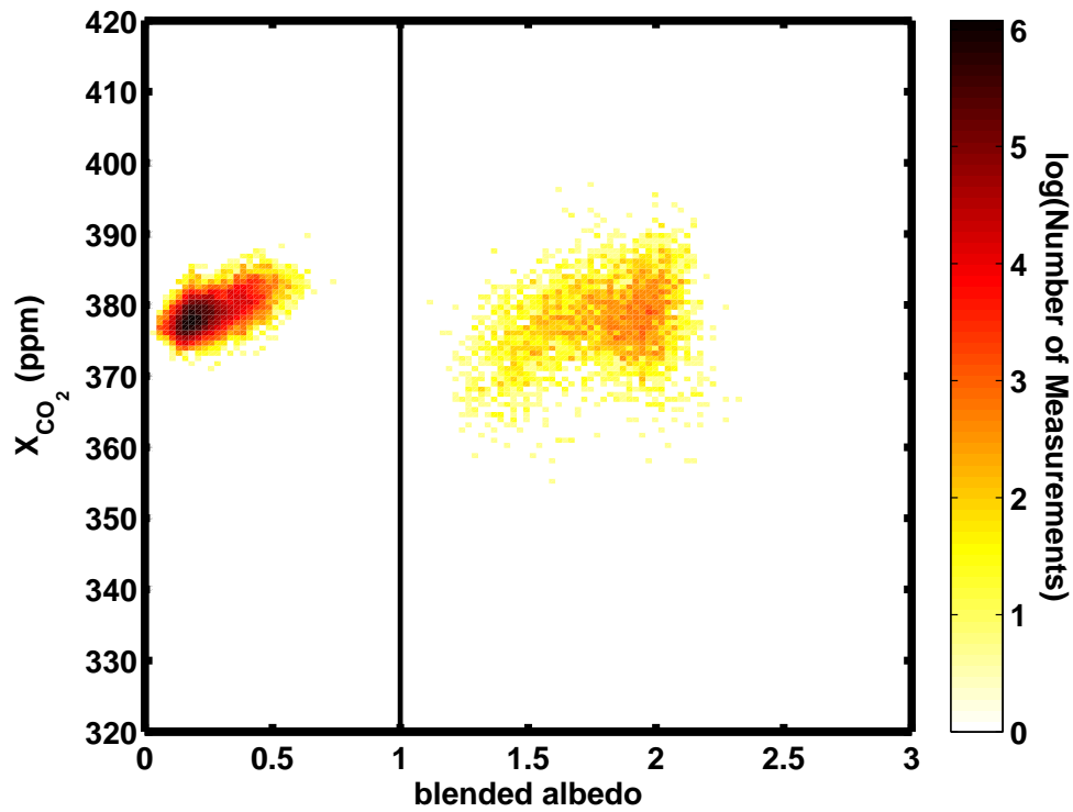
Fig. 4. An illustration of how snowy or icy scenes affect the ACOS-GOSAT data. There are two clear populations of points, delineated by a value of 1 in blended albedo (defined in Eq. 2 of the main text). Points to the left of the line at 1 are not influenced by snow and ice, and they are retained; points to the right are discarded. The colours represent the logarithm of the number of measurements in each 0.7 ppm by 0.025 units of blended albedo. The data in this figure are from soundings poleward of 25°S and span April 6, 2009 through March 21, 2011.
