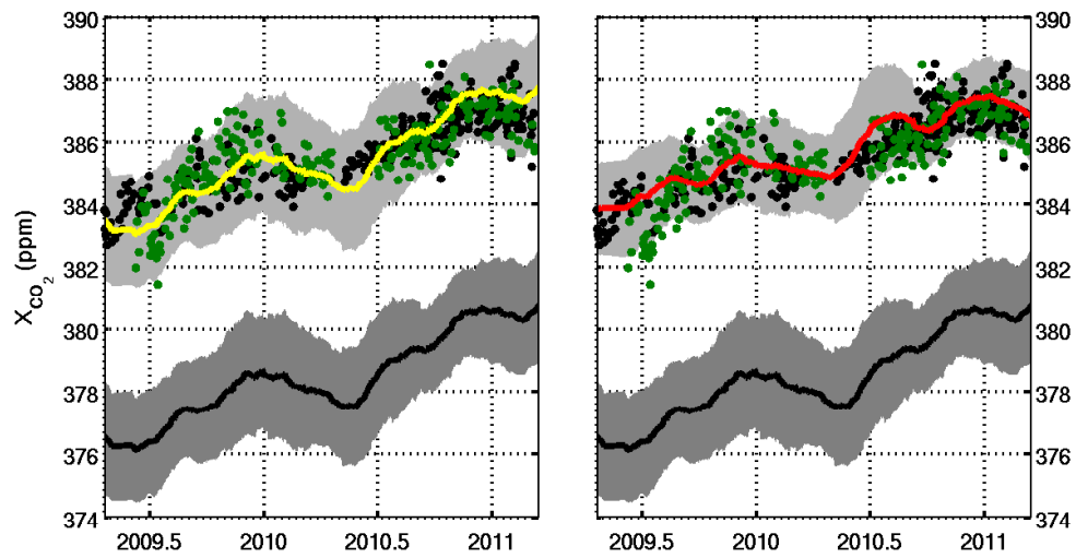
Fig. 5. The black curve is the original, unmodified ACOS-GOSAT data between 25^{\circ} S and 55^{\circ} S in both panels. The global bias (0.982) between the ACOS-GOSAT and TCCON data is removed in the left panel to obtain the yellow curve, and Eq. (4) is applied to obtain the red curve in the right panel. The grey shading represents 1\sigma . The TCCON data from Lauder, New Zealand (black circles) and Wollongong, Australia (green circles) are plotted for comparison.
