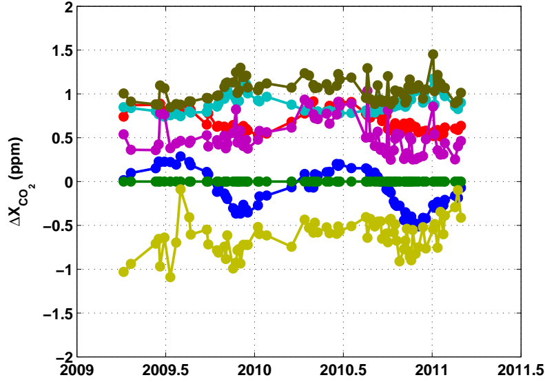
Fig. 8. The curves in this figure show the effect of the choice of a priori profile, and the effect of smoothing by the averaging kernels for data measured over the Lamont TCCON site. Plots show the ACOS-GOSAT adjustment to the ensemble profile ( \sum_j h_j (\mathbf{a}_1 - \mathbf{u})_j^T (\mathbf{x}_{a1} - \mathbf{x}_c)_j , blue), the TCCON adjustment to the ensemble profile ( \sum_j h_j (\mathbf{a}_2 - \mathbf{u})_j^T (\mathbf{x}_{a2} - \mathbf{x}_c)_j = 0 , green), the smoothing error ( \sqrt{\sum_k \sum_j h_j (\mathbf{a}_1 - \mathbf{a}_2)_j^T (\mathbf{S}_c)_{jk} (\mathbf{a}_1 - \mathbf{a}_2)_k} , red), the ACOS-GOSAT standard deviation ( \sigma_1 , cyan), the TCCON standard deviation ( \sigma_2 , purple), the difference between the TCCON adjusted ACOS-GOSAT smoothed values ( \hat{c}'_{12} - \hat{c}'_2 , yellow) and the square root of the sum of the TCCON and ACOS-GOSAT variances ( \sqrt{\sigma_1^2 + \sigma_2^2} , dark green). All parameters are defined in Appendix A.
