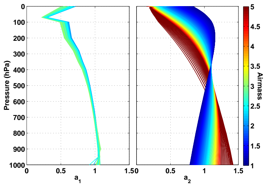
Fig. A2. Column averaging kernels for ACOS-GOSAT (left panel) and TCCON (right panel), coloured by the air mass. The GOSAT air mass range plotted here is much smaller than the range of TCCON air masses.
