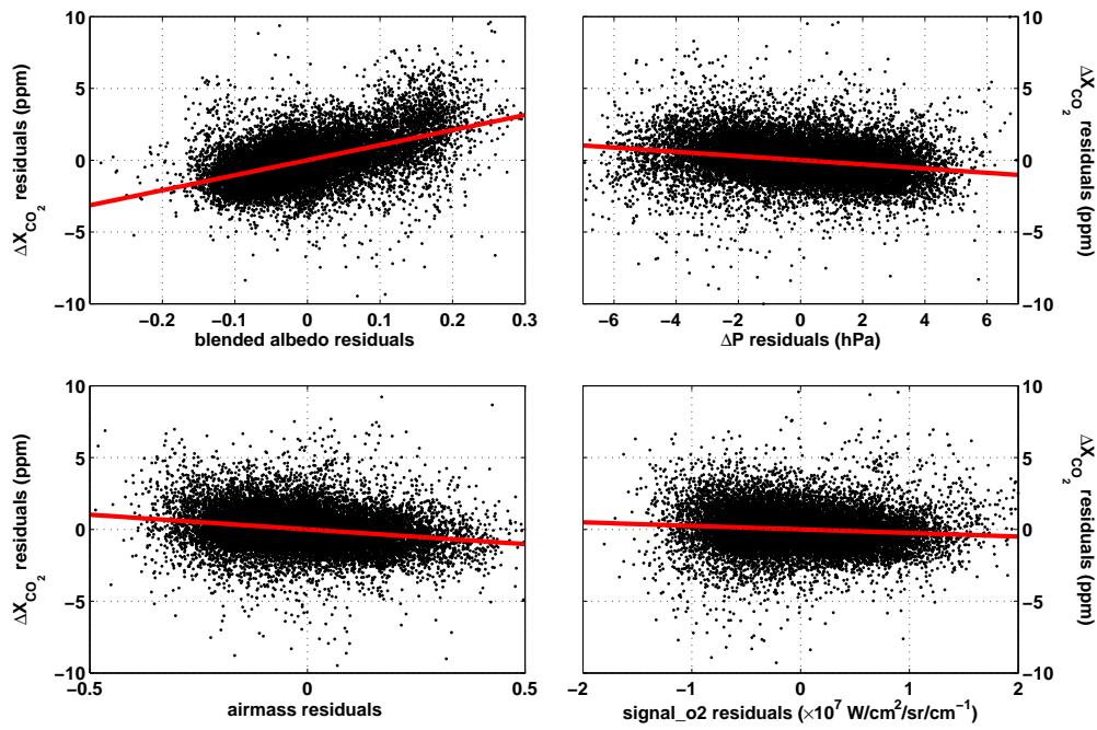
Fig. 6. Scatter plots showing the individual relationships between \Delta X_{\text{CO}_2} and the covariates simultaneously fitted in Eq. (4). These are data only from the Southern Hemisphere, where there should be no significant X_{\text{CO}_2} variations. The solid red lines are the best fit lines described by the coefficients listed in Table 2.
