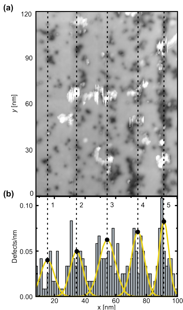
Figure 2: Helium ion induced line patterns in single layer MoS 2 . (a) STM topography of HIM patterned single layer MoS 2 . The ion-induced defects are arranged in a vertical line array with a pitch of 20 nm (black dashed lines), as expected. Ion dose and corresponding defect density increase towards the right. The most apparent defects (type A) appear as dark depressions. White, streaky areas correspond to surface adsorbates. (b) Spatial distribution of HIM induced defects. Yellow lines are Gaussian fits, black dashed lines indicate the fitted mean. Imaging parameters: V_b = 0.5 V, I_t = 100 pA, 100 nm x 120 nm.
