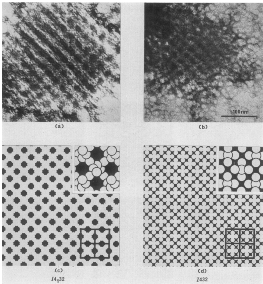
PLATE II. (a) and (b) Fragments of form I RuDPCase crystals, negatively stained in uranyl acetate. Magnification 200,000\times .
