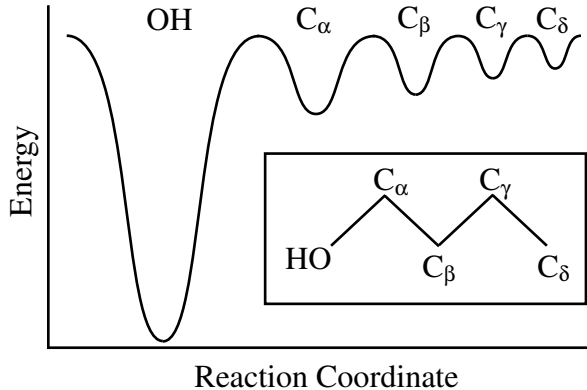
Figure 4: One-dimensional potential energy surface used in the simulation of rearrangement dynamics for \text{Cr}(\text{CO})_6 in butanol. All other alcohol solutions have the same form of the potential energy surface and vary only in the number and depth of the various wells.
