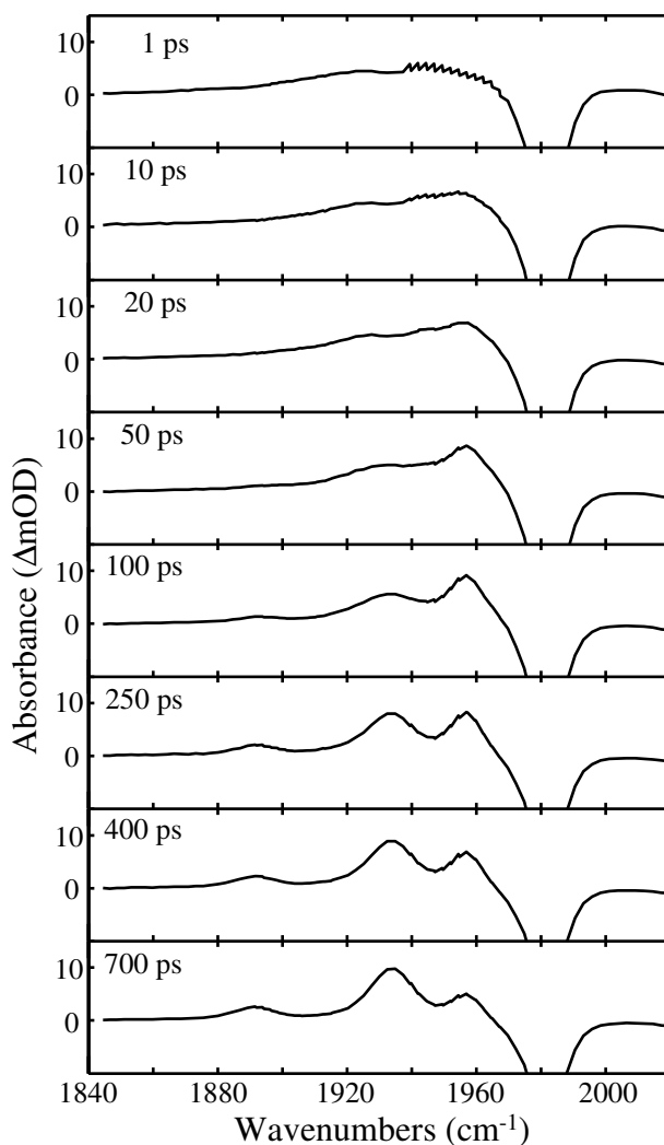
Figure 7: UV-pump, IR-probe spectra of chromium hexacarbonyl in neat 1-butanol at increasing delay times after photoexcitation.
