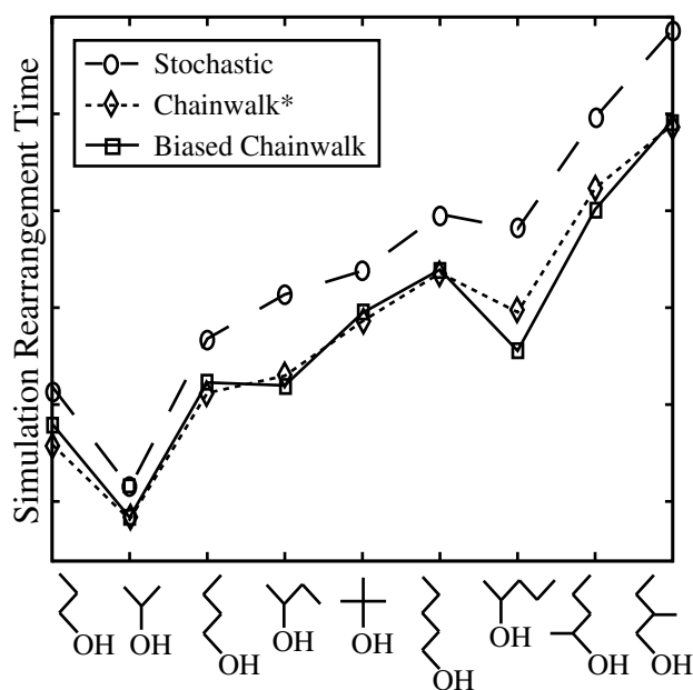
Figure 13: Simulation data for all alcohol solvents. *Note that the chainwalk simulation times have been divided by 2 to allow for comparison of the trend.
