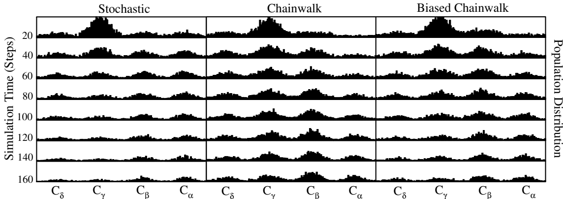
Figure 14: Evolution of population distribution at increasing times after starting at the center of the C_\gamma well of 1-butanol. Each distribution shown is 20 simulation steps after initialization. Loss of population from the alkyl wells (shown) is transferred into the hydroxyl well (not shown).
