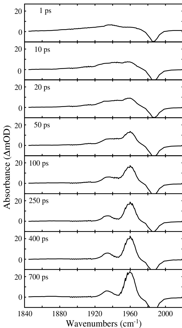
Figure 6: UV-pump, IR-probe spectra of chromium hexacarbonyl in neat pentane at increasing delay times after photoexcitation.
