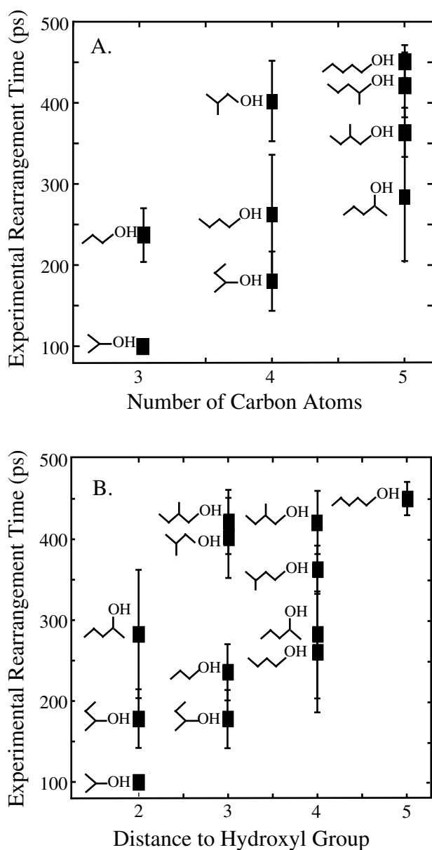
Figure 9: Experimental rearrangement times grouped according to the number of carbon atoms in the alcohol (A) and according to the distance from the end of the alkyl chain to the hydroxyl site (B).
