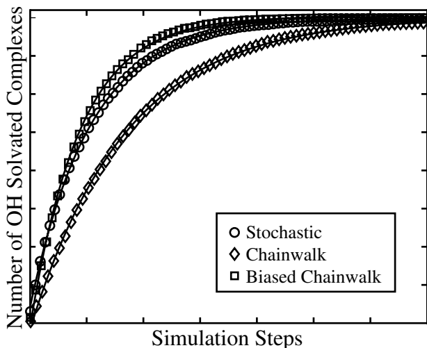
Figure 11: Simulation kinetic traces for \text{Cr}(\text{CO})_5 in 1-butanol. Circles represent stochastic simulation results, diamonds represent chainwalk results, and squares represent biased chainwalk results. Single exponential fits are overlaid onto the data.
