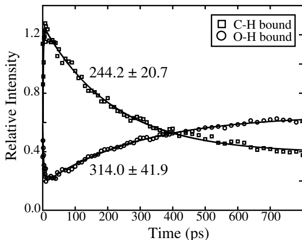
Figure 8: Experimental kinetic data for chromium hexacarbonyl in 1-butanol. Kinetic traces of the alkyl bound complex (open squares) and the hydroxyl bound complex (open circles) are shown with single exponential fits to the data (solid lines). Time constants for the exponential fits are shown beside each trace.
