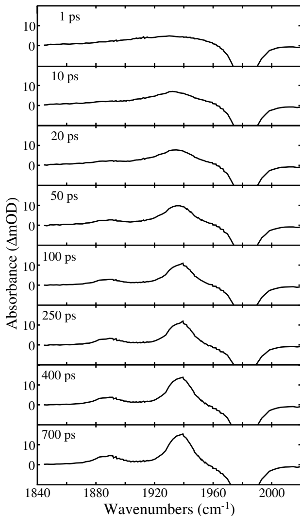
Figure 5: UV-pump, IR-probe spectra of chromium hexacarbonyl in neat methanol at increasing delay times after photoexcitation.
