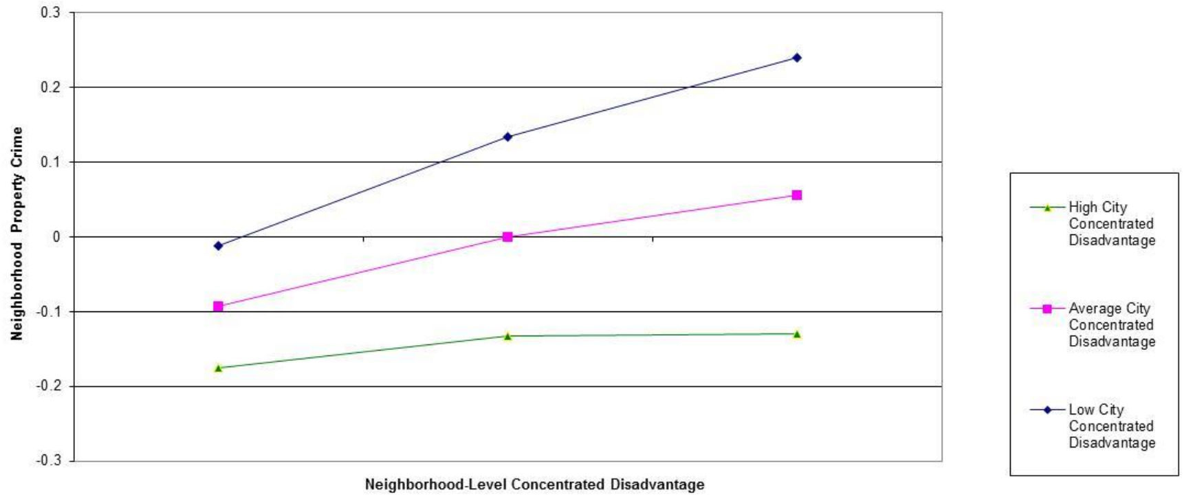
Figure 2: Effect of interaction of Neighborhood Concentrated Disadvantage and City Concentrated Disadvantage on Neighborhood Property Crime
