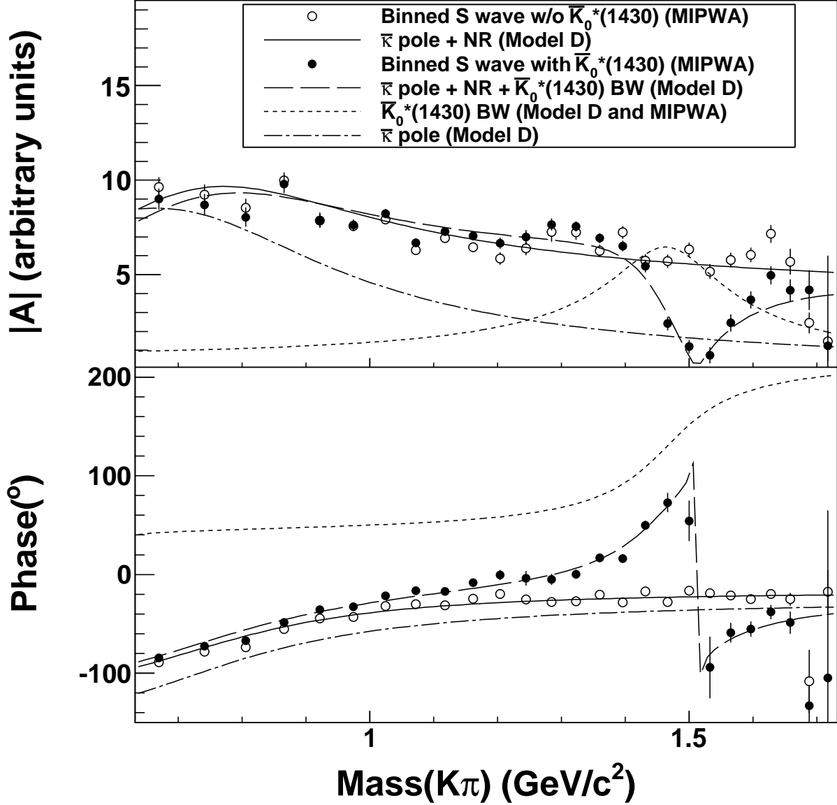
Figure 7. The magnitude and phase of the K\pi S -wave in model D and the MIPWA. The open circles with error bars (statistical uncertainties only) show the binned K\pi S -wave without the \bar{K}_0^*(1430) and the black dots show the total K\pi S -wave. Other curves show the S -wave components of model D.
