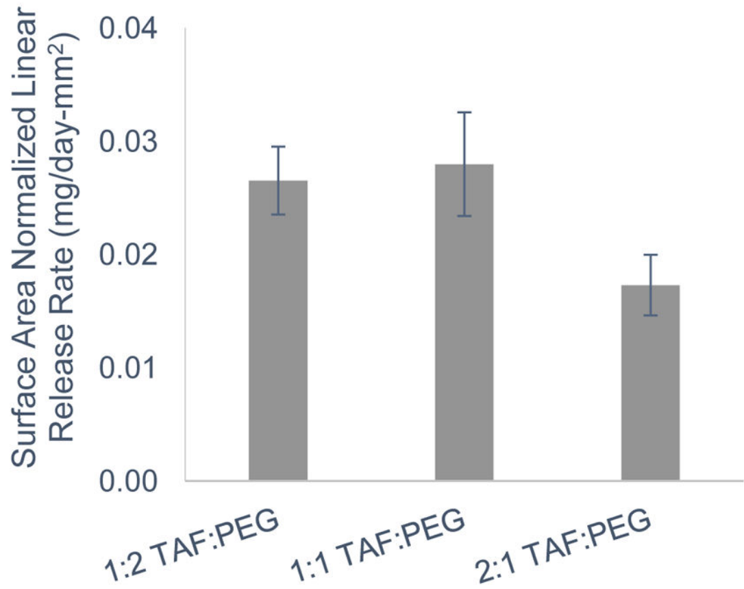
Figure 4. Reference source not found.: Surface area normalized release rates for TAF from PCL TFPD (8.5 \mu\text{m} membrane) with a range of w/w ratios of TAF to PEG300. No statistically significant difference in release rates ( p=0.16 ).
