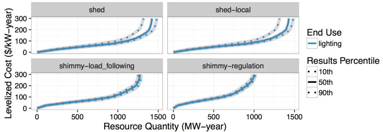
Figure 78: Commercial Lighting end-use level supply curves.
