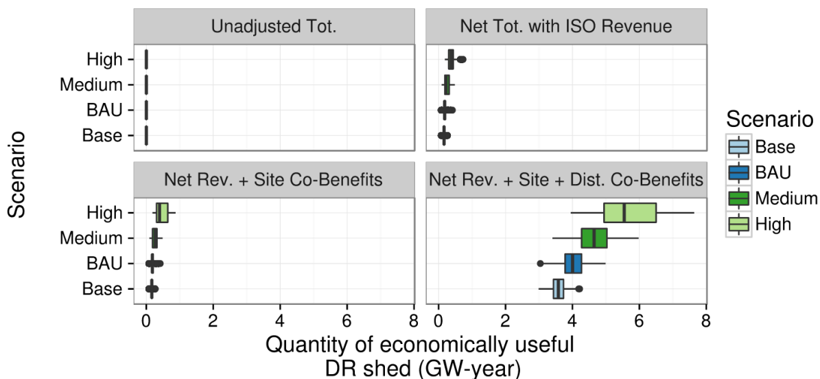
Figure 64: Box plots depicting the 2025 Shed-type DR potential as compared to the system-level value from the levelized demand curves.
