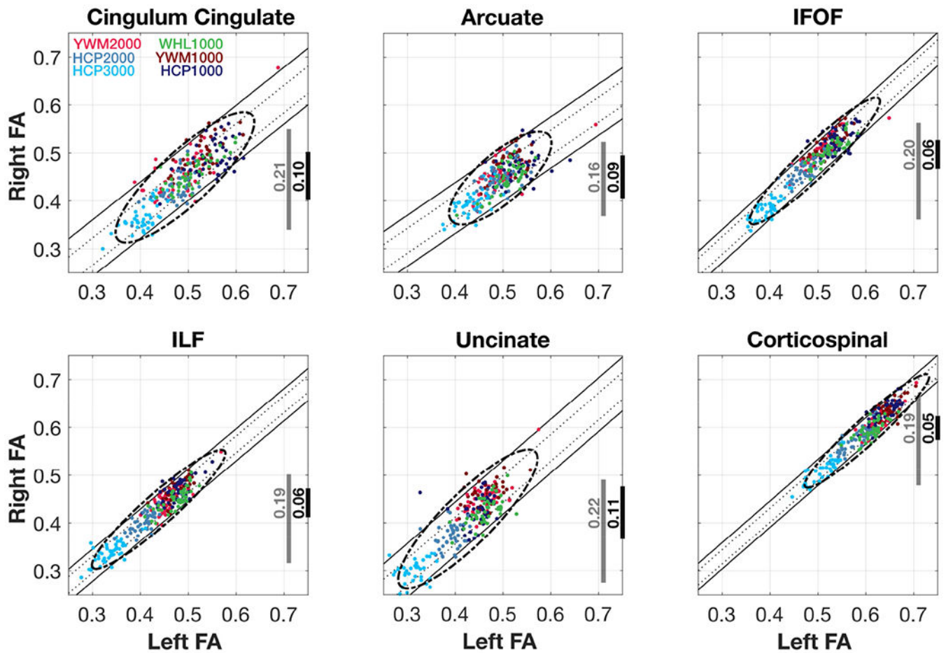
Figure 7. Homologous tract Left-Right FA scatterplots and iso-residual contour lines Scatterplot of the Left-Right mean FA for all tracts and all projects. The grey vertical lines shows the 95% range of all Right FA values, and the black line the range of possible values for any given Left FA value. The diagonal bands are the iso-residual contour lines holding the 68% and 95% of the residuals from the linear model fitted to all the six datasets.
