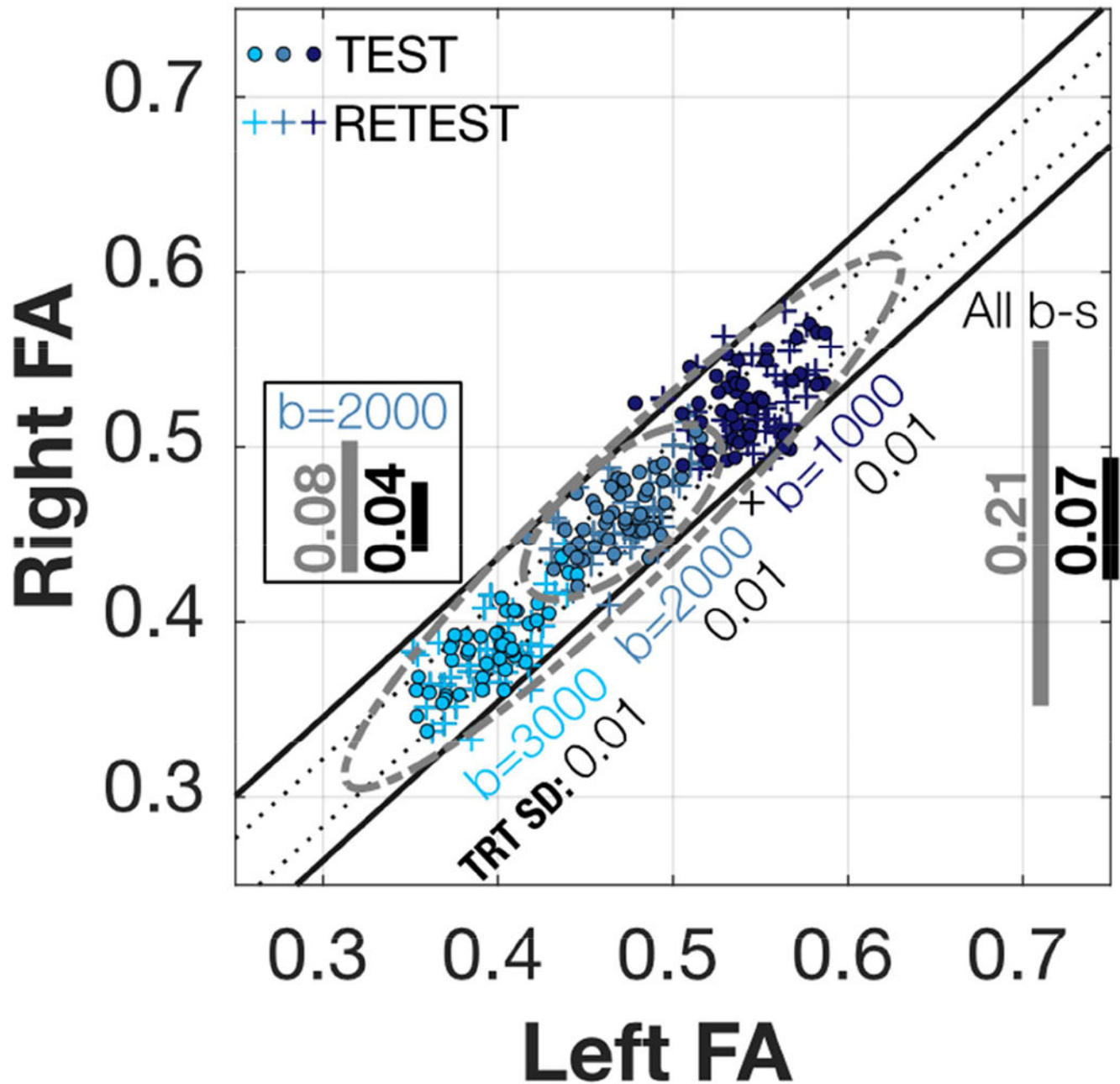
Figure 6. Left-Right IFOF FA scatterplots and iso-residual contour lines for HCP
