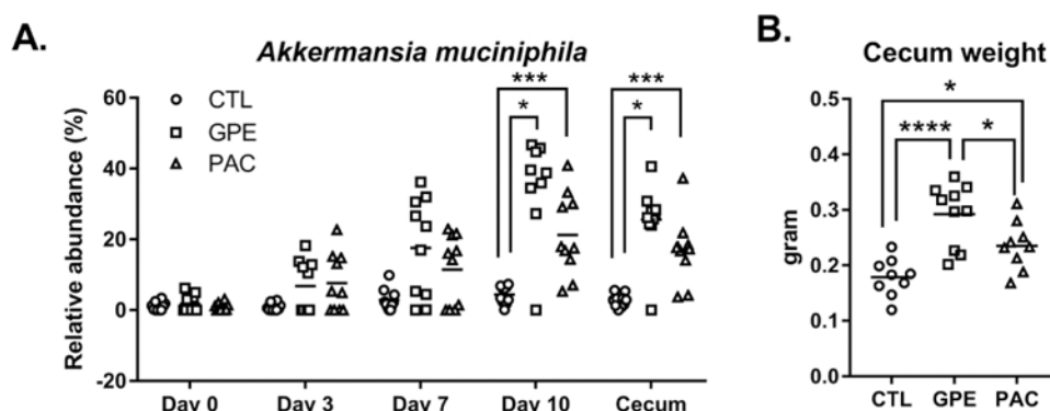
Figure 4. Comparison of PAC vs. GPE treatment on A. muciniphila bloom and cecal weight
