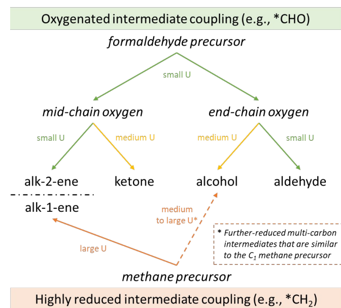
Fig. 9 General hypotheses regarding the eCO 2 R mechanism.
