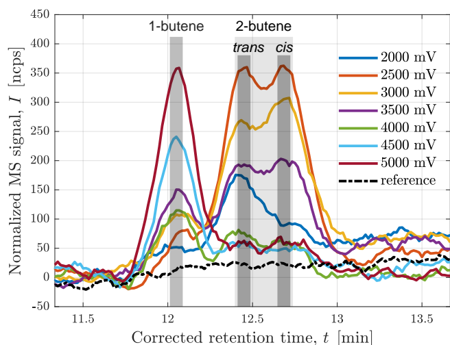
Fig. 2 Extracted ion chromatogram for m/z = 57.070\text{Da} ( \text{C}_4\text{H}_9^+ ion) from experiments at different applied potentials U_{\text{Hg}/\text{HgO}} compared to a reference measurement without copper-based catalyst.
