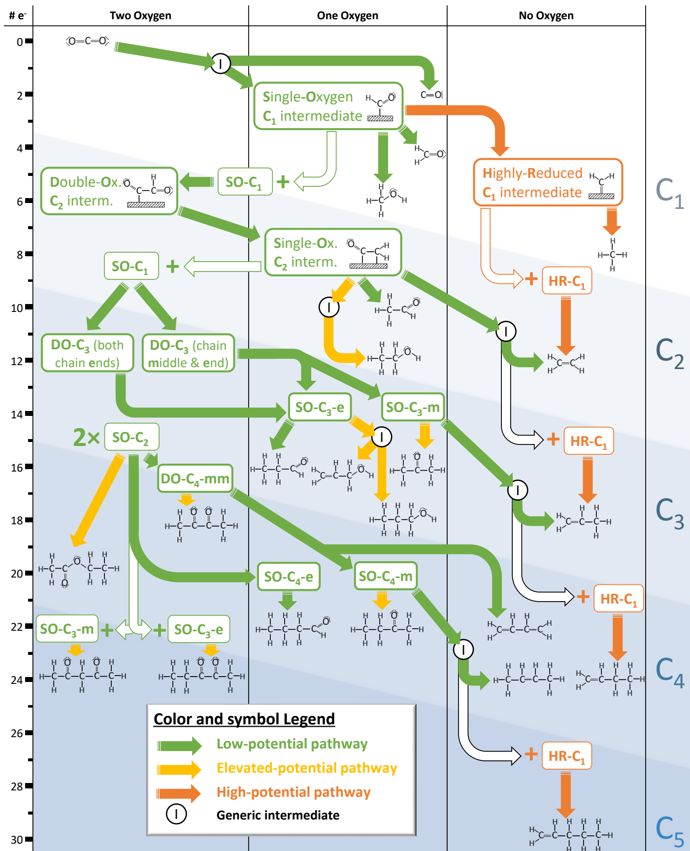
Fig. 8 Overview of identified electrocatalytic \text{CO}_2 reduction products, supplemented by the reaction mechanism hypothesized in this study and likely key intermediates. Names given for suspected intermediates are based on reduction state (highly-reduced vs. single- or double-oxygenated), chain length ( \text{C}_1 - \text{C}_5 ), and position of oxygen if applicable (mid-chain vs. end-chain). The separation by number of carbon and oxygen as well as number of electrons transferred makes this graph a useful template for further mechanism discussion in the form established by Nitopi et al. 3 .
