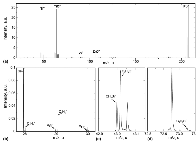
Figure 2. High spectra resolution ToF-SIMS investigations of the PZT surface after scanning with an AFM tip. (a) Total ion mass spectrum; (b–d) zoomed-in plots of (b) \text{Si}^+ isotopes, (c) \text{CH}_3\text{Si}^+ , and (d) \text{C}_3\text{H}_9\text{Si}^+ peaks.
