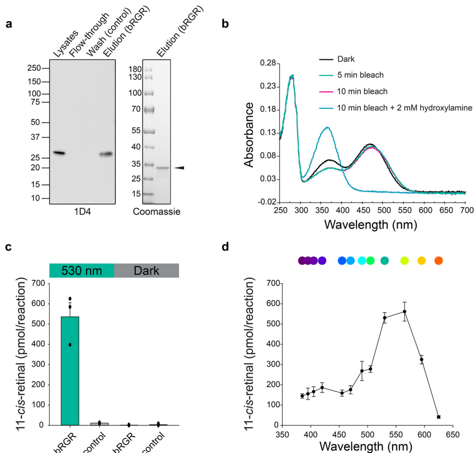
Figure 8. Photoisomerase activity of immunopurified bovine RGR expressed in HEK293S GnTI - cells. a , immunoblot of purified bRGR detected by 1D4 antibody (left). Coomassie-stained SDS-polyacrylamide gel of purified bRGR (right). b , absorption spectra for purified bRGR bound to all-trans-retinal. The spectrum of bRGR was measured in the dark and after 5 and 10 min of illumination with 530 nm light. Excess hydroxylamine was then added, and the spectrum of the sample was measured again. c , amounts of 11-cis-retinal produced from all-trans-retinal by purified bRGR in a photoisomerization assay. Control sample consists of the immunochromatography elution buffer. n = 3 for each group. Data are shown as mean \pm S.E. d , action spectrum showing the amounts of 11-cis-retinal photoisomerized from all-trans-retinal by purified bRGR during 30 min of light exposure with the given wavelength and a fixed intensity at 400 \mu W. n = 4 for the 530 and 565 nm, n = 3 for the other wavelengths. Data are shown as mean \pm S.E.
