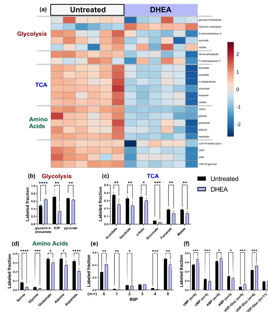
Figure 6. DHEA (G6PD inhibitor) decreased the ^{13}\text{C} enrichments of HUVEC glycolytic and TCA metabolites, as well as amino acids, R5P, and nucleotide precursors UMP and AMP. (a) Heatmap comparing ^{13}\text{C} metabolite enrichment of untreated HUVECs and DHEA-treated HUVECs. ^{13}\text{C} enrichment of (b) glycolytic metabolites, (c) TCA metabolites, (d) amino acids, (e) R5P, and (f) UMP, AMP, and UDP-glucose. Statistical significance for (b–f) determined through Welch’s unequal variances t -test; * p < 0.05 , ** p < 0.01 , *** p < 0.001 , **** p < 0.0001 . n = 6 biological replicates.
