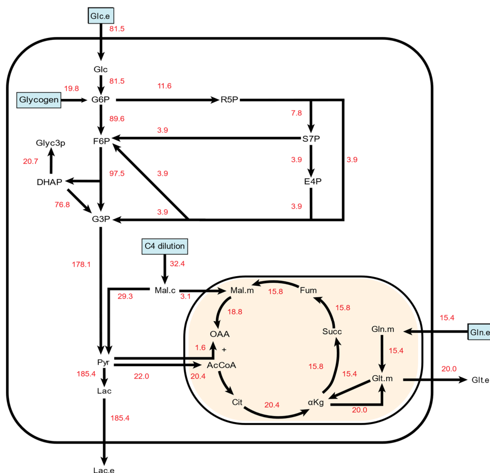
Figure 2. A simplified metabolic flux map depicting net metabolic fluxes in untreated HUVECs. All numbers are given in nmol/cells/hr. Carbon sources in the final model are indicated in light blue boxes. To simplify PPP pathway visualization, only the unique metabolites formed in each reaction are depicted along with the net PPP-based production of F6P and G3P. Full information on reaction schemes, atom transition specifications, and fluxes can be found in Supplemental File S1.
