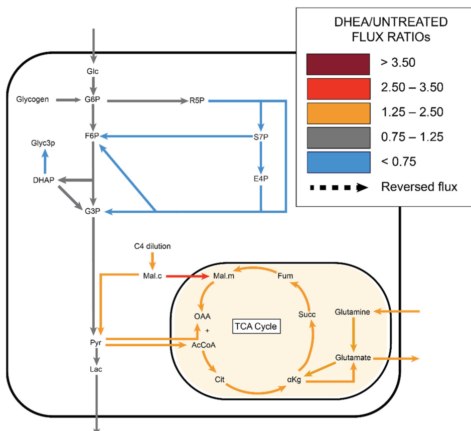
Figure 7. ^{13}\text{C} MFA estimated decreased non-oxidative PPP flux with increased TCA flux in DHEA (G6PD inhibitor) treated cells, with the malate shuttle importing malate from cytoplasm to mitochondria.
