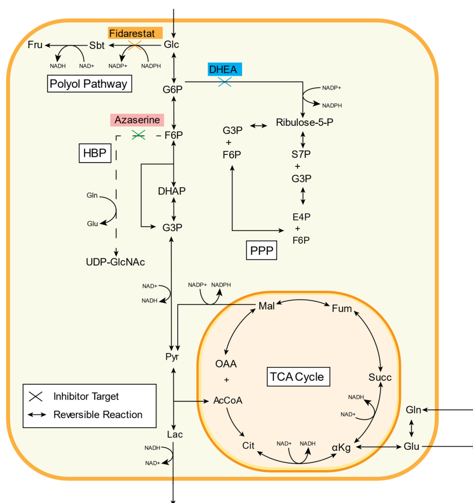
Figure 1. Three inhibitors (fidarestat, dehydroepiandrosterone (DHEA), and azaserine) were used to decrease glucose flux down glycolytic side branch pathways (polyol, PPP, and HBP, respectively). Fidarestat inhibits aldose reductase, an enzyme that catalyzes the first rate-limiting step of the polyol pathway and reduces glucose to sorbitol. DHEA inhibits glucose-6-phosphate dehydrogenase (G6PD), an enzyme involved in converting glucose-6P into 6P-glucolactone in the PPP. Azaserine inhibits the rate-limiting enzyme GFAT in the HBP, a pathway responsible for producing UDP-GlcNAc. See Table 1 for metabolite abbreviations.
