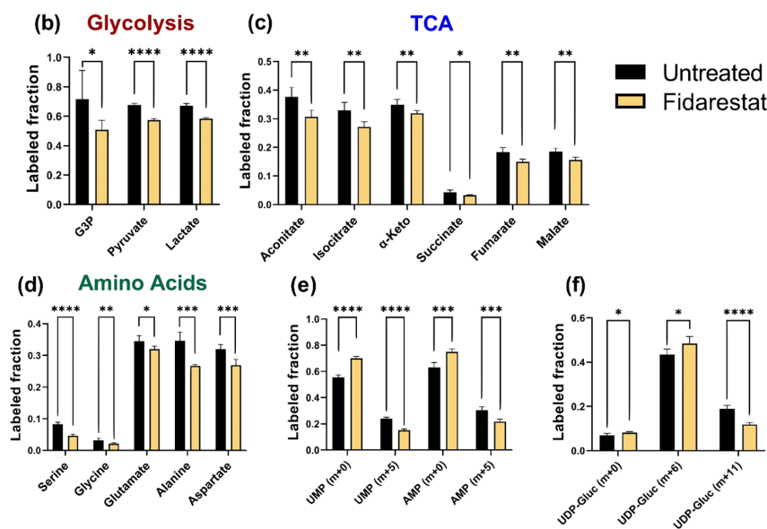
Figure 4. Fidarestat (aldose reductase inhibitor) decreased the 13 C enrichments of HUVEC glycolytic and TCA metabolites, as well as amino acids, nucleotide precursors, and UDP-glucose. (a) Heatmap comparing 13 C metabolite enrichment of untreated HUVECs and fidarestat-treated HUVECs. 13 C enrichment of (b) glycolytic metabolites, (c) TCA metabolites, (d) amino acids, (e) AMP and UMP, and (f) UDP-glucose. Statistical significance for (b–f) determined through Welch’s unequal variances t -test; * p < 0.05; ** p < 0.01; *** p < 0.001; **** p < 0.0001. n = 6 biological replicates.
