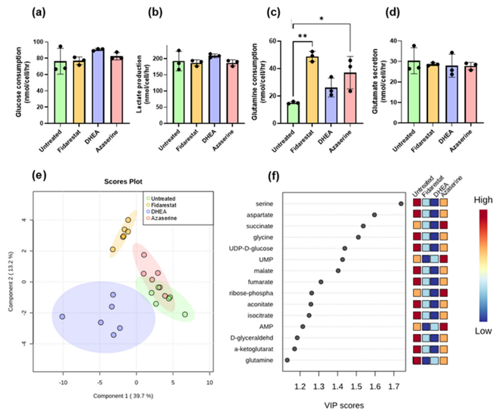
Figure 3. Fidarestat (aldose reductase inhibitor), DHEA (G6PD inhibitor), and azaserine (GFAT inhibitor) only changed external fluxes for glutamine consumption; however, fidarestat and DHEA-treated cells clustered separately from untreated cells by PLS-DA, with amino acids and TCA metabolites explaining most of the differences. (a) glucose consumption, (b) lactate secretion, (c) glutamine consumption, and (d) glutamate secretion all measured by YSI bioanalyzer after 24 h of inhibitor treatment. (e) PLS-DA clustering of total enrichment data. (f) VIP scores plot showing metabolites that significantly contributed to PLS-DA class discrimination. Results in (a–d) are mean \pm s.d. with n = 3 biological replicates. Results in e and f are n = 6 biological replicates. Statistical significance was determined with one-way ANOVA followed by Dunnett’s multiple comparison test. * p < 0.05 ; ** p < 0.01
