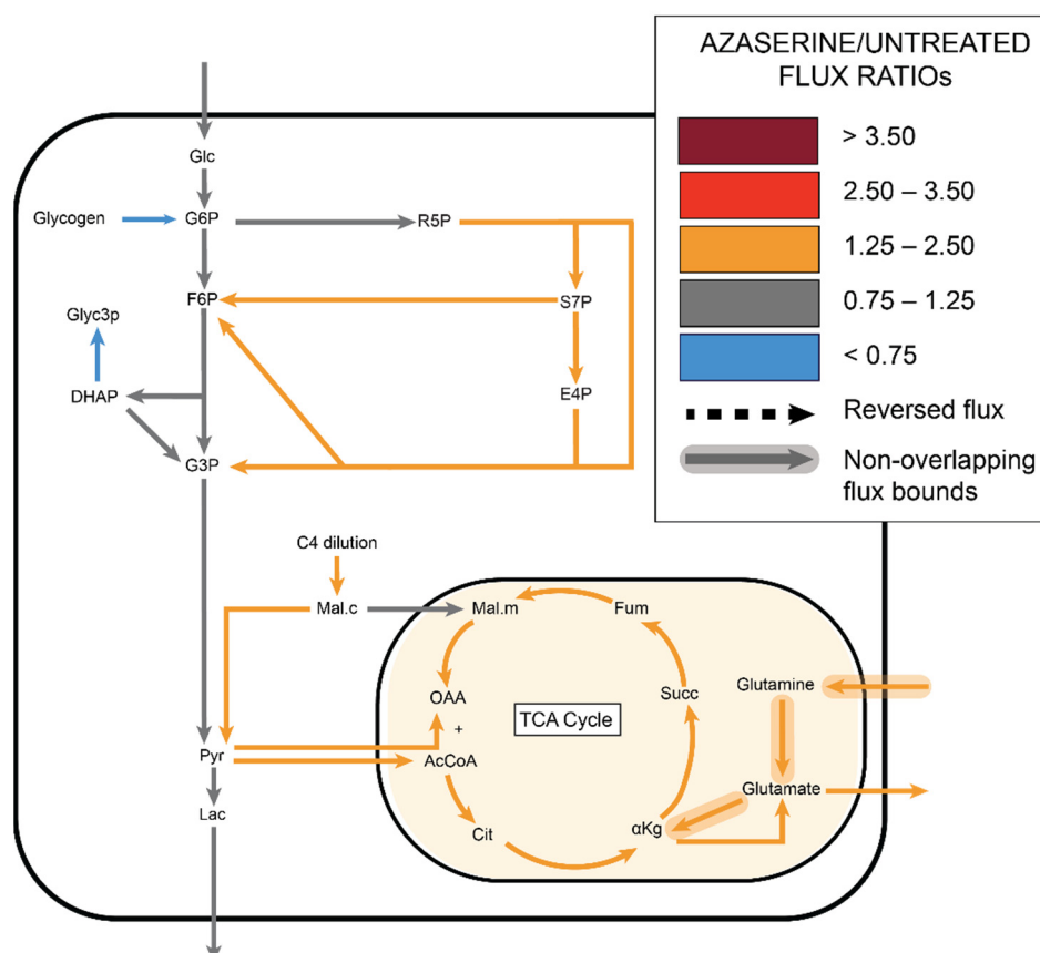
Figure 9. ^{13}\text{C} MFA estimated increased non-oxidative PPP flux with increased TCA flux in azaserine (GFAT inhibitor) treated cells.
