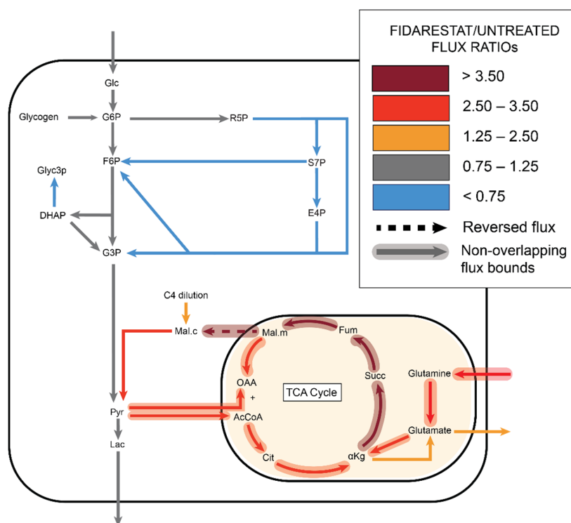
Figure 5. 13 C MFA estimated decreased non-oxidative PPP flux with increased TCA flux in fidarestat (aldose reductase inhibitor) treated cells, with the malate shuttle exporting malate from mitochondria to cytoplasm.
