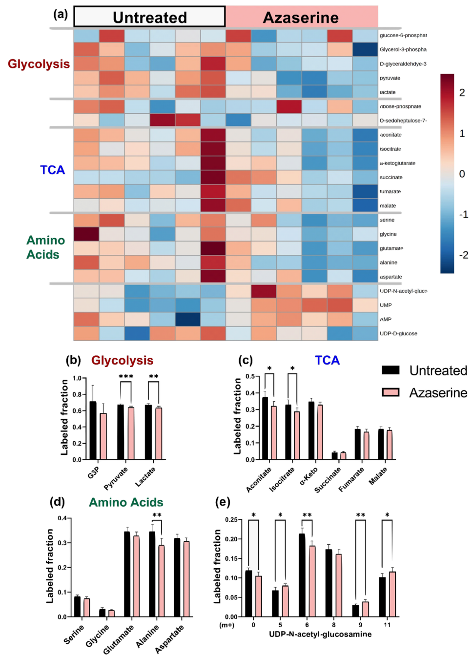
Figure 8. Azaserine (GFAT inhibitor) decreased the ^{13}\text{C} enrichments of HUVEC glycolytic metabolites and had varied effects on TCA metabolites, amino acids, and UDP-GlcNAc. (a) Heatmap comparing ^{13}\text{C} metabolite enrichment of untreated HUVECs and azaserine-treated HUVECs. ^{13}\text{C} enrichment of (b) glycolytic metabolites, (c) TCA metabolites, (d) amino acids, and (e) UDP-GlcNAc. Statistical significance for (b–f) determined through Welch’s unequal variances t -test; * p < 0.05 ; ** p < 0.01 ; *** p < 0.001 . n = 6 biological replicates.
