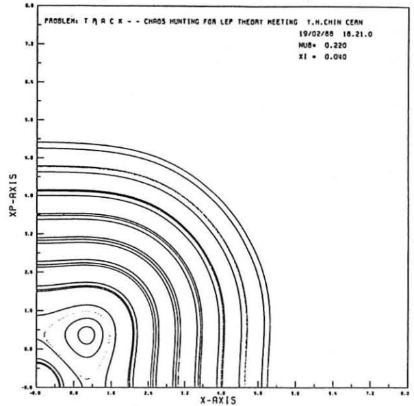
Fig. 1(a) One quarter of phase-space trajectories for v_\beta = 0.22 and \xi = 0.04 .
