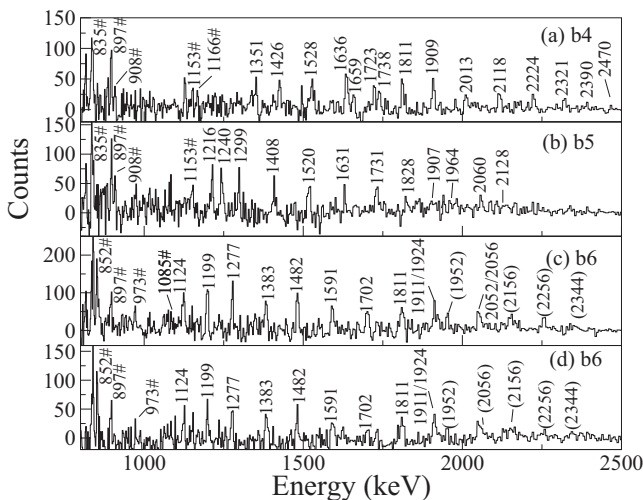
FIG. 3. Summed triple-gated \gamma -ray coincidence spectra of bands b4–b6 in ^{124}\text{Xe} . The spectra in panels (a)–(c) were produced by triple gates on all transitions of bands b4, b5, and b6, respectively. The triple-gated spectrum in panel (d) was obtained with a single gate on the 2052-keV transition and a combination of two gates on all the transitions of band b6. Transitions marked by # signs in panels (a)–(d) stem from low-energy levels which receive the highest-intensity feeding from bands b4–b6.
