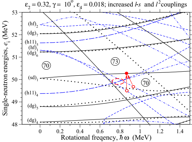
FIG. 14. Calculated neutron orbitals at the same deformation as in Fig. 12, but with the l \cdot s and l^2 strengths in the \mathcal{N} = 5 oscillator shell increased by approximately 20% relative to the A = 110 parameters [25]. Band b4 is assigned to the configuration with all orbitals below the Z = 70 gap at \hbar\omega \approx 1.0 MeV occupied, while one particle is lifted to the \alpha = 1/2 (sd)_1 orbital according to the arrows in bands b3 and b6. For lower frequencies in these bands, the odd (hf)_1 particle moves to the (h11)_4 orbital, where these orbitals cross within the ellipse drawn by a dashed line.
