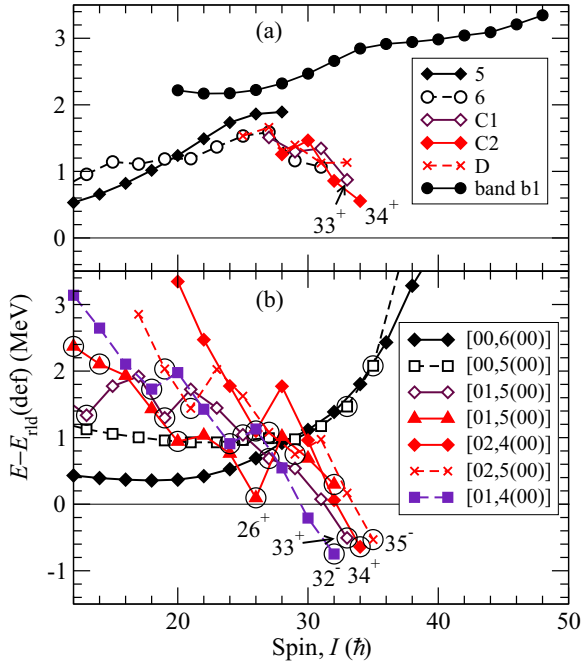
FIG. 9. Excitation energies, relative to a rotating liquid-drop energy, for observed (a) and calculated (b) valence-space states in ^{124}\text{Xe} . Calculated states with spin vectors aligned along the oblate symmetry axis are highlighted by large open circles; states corresponding to experimentally observed levels are labeled by their spins.
