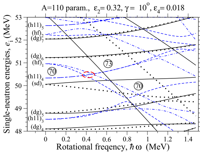
FIG. 12. Calculated neutron orbitals as a function of rotational frequency, \hbar\omega , at a deformation typical for the high-spin configurations of ^{124}\text{Xe} , \epsilon_2 = 0.32 , \gamma = 10^\circ , \epsilon_4 = 0.018 . The orbitals are labeled at \hbar\omega = 0 by their dominant j -shell amplitude and the ordering within the respective groups. The h_{11/2} orbitals are labeled as (h11) while pseudospin partners [31] d_{5/2}g_{7/2} , s_{1/2}d_{3/2} , and h_{9/2}f_{7/2} are labeled as (dg) , (sd) , and (hf) , respectively. Dashed (or dot-dashed) lines are used for negative-parity orbitals while lines with dots are used for signature \alpha = -1/2 . The crossing between the (h11)_4 and (hf)_1 orbitals is highlighted with a dashed ellipse.
