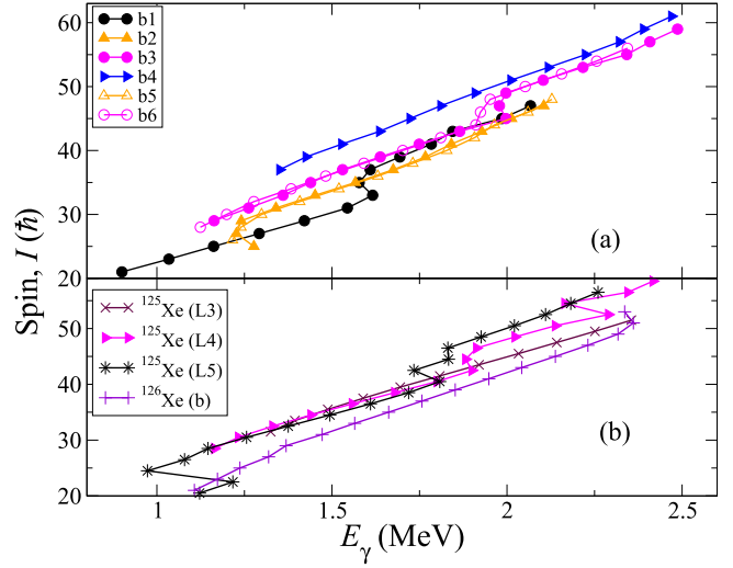
FIG. 7. Spins of states as a function of \gamma -ray energies depopulating these states for (a) ^{124}\text{Xe} , (b) ^{125}\text{Xe} [12], and ^{126}\text{Xe} [14].
