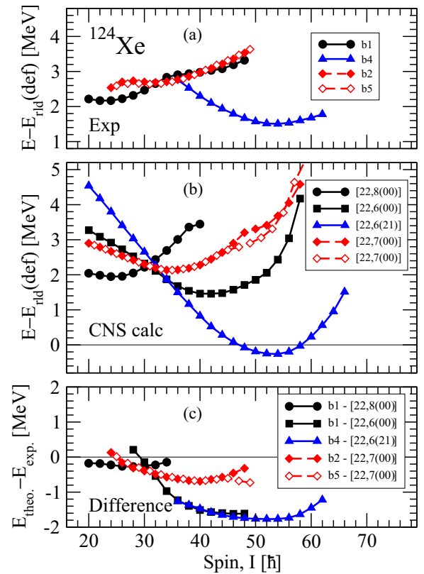
FIG. 13. Comparison between experiment and calculations for bands b1, b2, b4, and b5. Observed and corresponding calculated bands are drawn in panels (a) and (b), respectively, with the difference between calculations and experiment being given in panel (c). The convention for lines and symbols is the same as that in Fig. 11.
