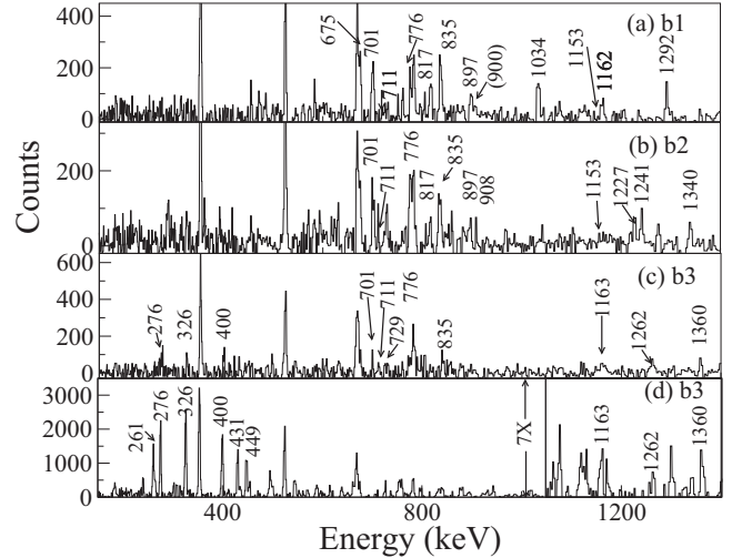
FIG. 4. Summed triple-gated \gamma -ray spectra showing \gamma -ray transitions from low-spin states observed in coincidence with transitions of the high-spin bands b1–b3 in ^{124}\text{Xe} . For panels (a)–(c), triple gates on all transitions of the respective bands were used. For panel (d), double gates on transitions of band b3 and a single gate on each of the transitions with energies 261, 276, 326, 400, 431, and 449 keV from sequences 3 and 4 were used. The higher-energy transitions of band b3 are shown in panel (d) on a magnified scale.
