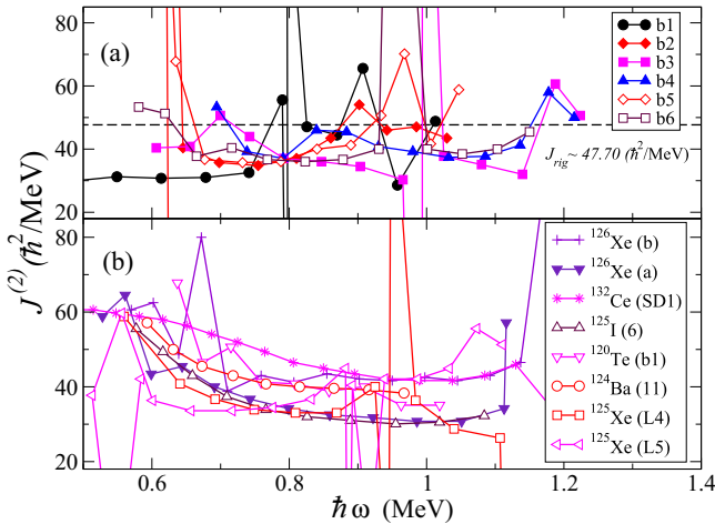
FIG. 6. (a) Dynamic moments of inertia, J^{(2)} , as a function of rotational frequency for the six new highly deformed bands in ^{124}\text{Xe} . (b) J^{(2)} vs rotational frequency for similar bands in ^{120}\text{Te} [7], ^{125}\text{I} [13], ^{125}\text{Xe} [12], ^{126}\text{Xe} [14], ^{124}\text{Ba} [5], and ^{132}\text{Ce} [23], respectively.
