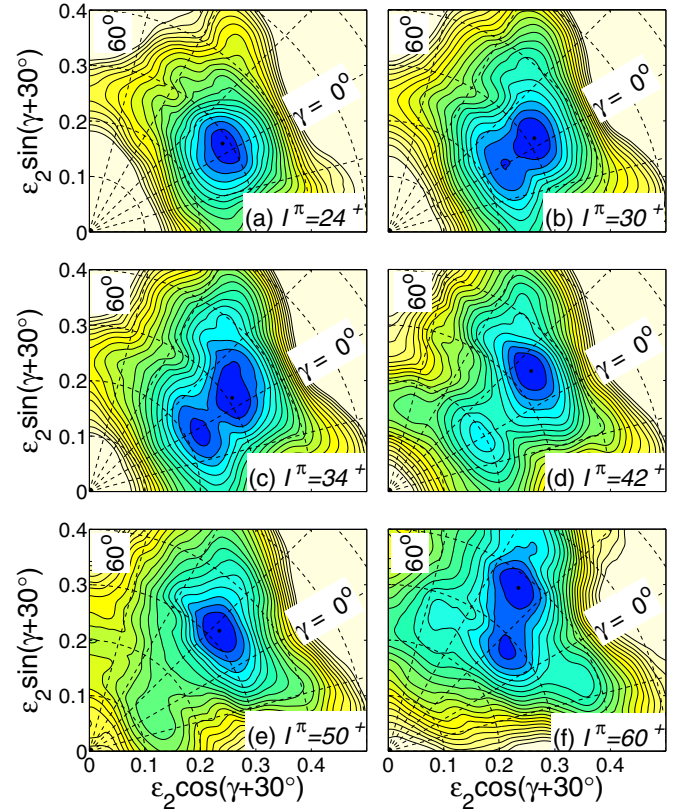
FIG. 10. Calculated total-energy surfaces for ^{124}\text{Xe} configurations with positive parity and even spins with the extra constraint of the presence of two proton holes in g_{9/2} orbitals. The contour-line separation is 0.25 MeV.
