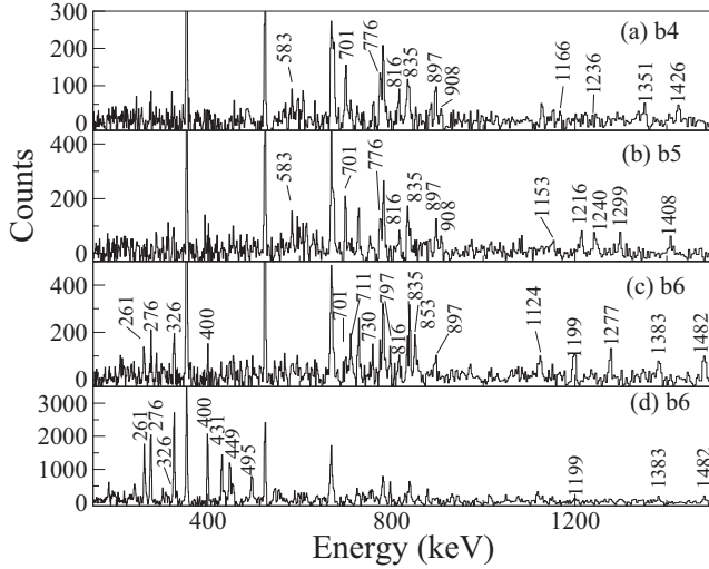
FIG. 5. Summed triple-gated \gamma -ray spectra showing \gamma -ray transitions from low-spin states observed in coincidence with transitions of the high-spin bands b4–b6 in ^{124}\text{Xe} . For panels (a)–(c), triple gates on all the transitions of the respective bands were used. For panel (d), double gates on transitions of band b6 and a single gate on each of the transitions with energies 261, 276, 326, 400, 431, and 449 keV from sequences 3 and 4 were used.
