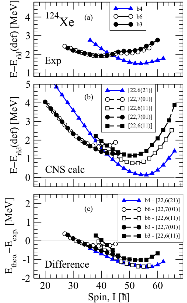
FIG. 15. Comparison between (a) experiment and (b) calculations for bands b4, b3, and b6. The calculated results were obtained with the new parameters of Fig. 14. The energy difference between experiment and calculation is shown in panel (c). The convention for lines and symbols is the same as that in Fig. 11.
