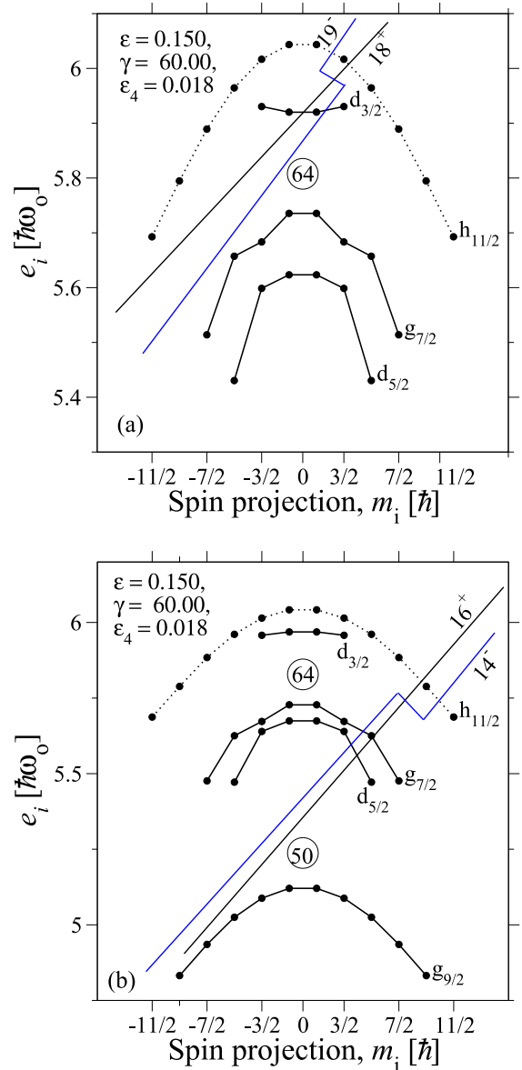
FIG. 8. Calculated single-particle energies, e_i , as a function of the spin-projection quantum number, m_i , at \varepsilon_2 \approx 0.15 , \gamma = 60^\circ : (a) for neutrons and (b) for protons. Some low-lying aligned configurations are defined by “straight-line Fermi surfaces,” where the orbitals below the lines are occupied and the total spin is obtained as the sum of the projections m_i below the lines.
