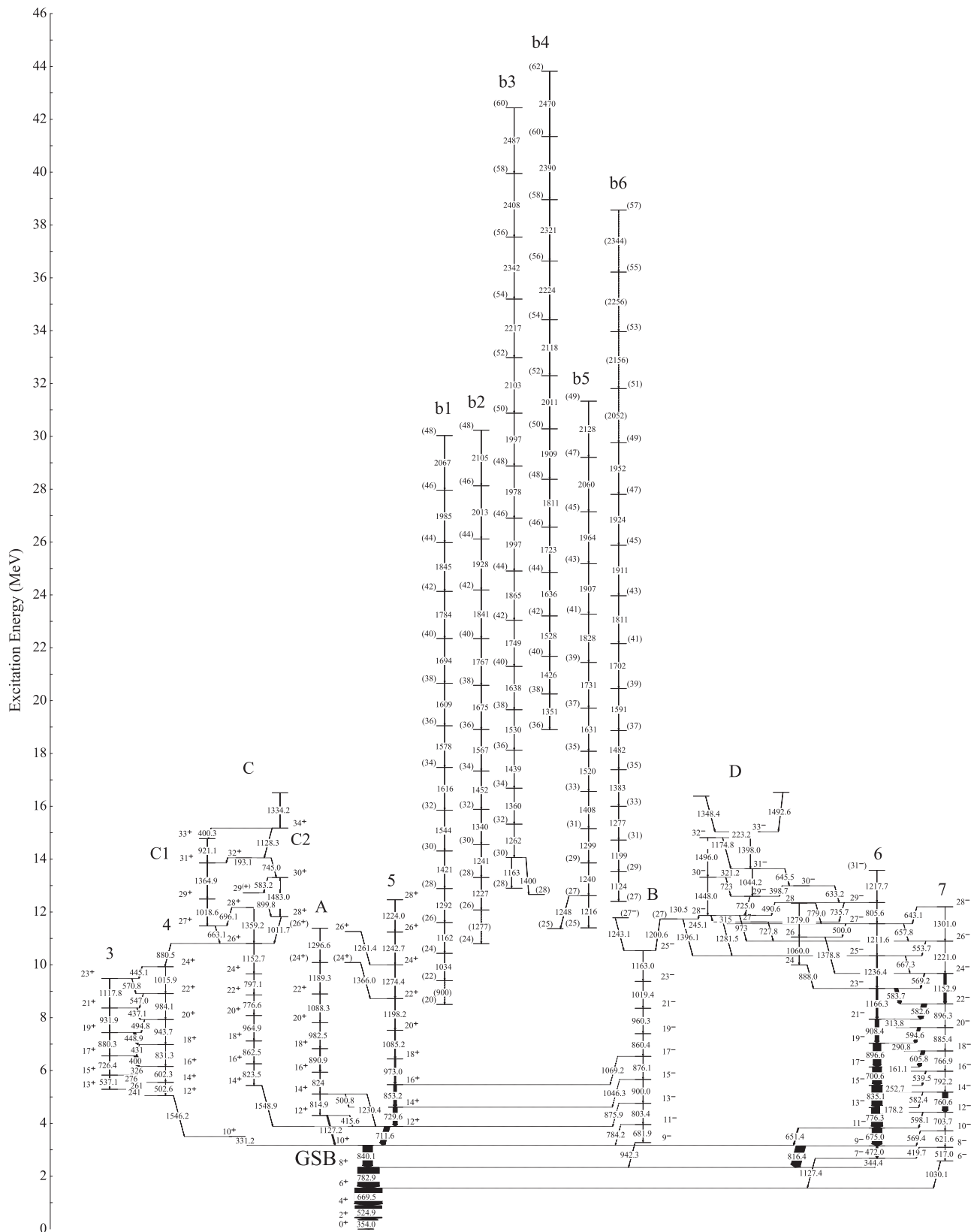
FIG. 1. A partial level scheme of ^{124}\text{Xe} . The low- and medium-spin states (structures 1–7 and A–D) have been adopted from Al-Khatib et al. [6]. The newly discovered bands are labeled b1–b6.
