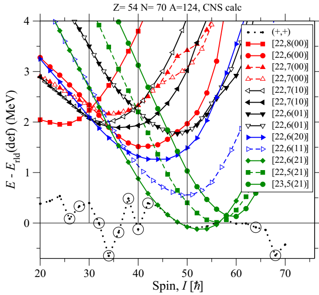
FIG. 11. Calculated excitation energies relative to a rotating liquid-drop energy vs spin for some of the lowest-energy configurations in ^{124}\text{Xe} with two protons excited from the g_{9/2} subshell below the Z = 50 gap. Configurations with the same number of neutrons excited across the N = 82 gap are drawn with the same color. The positive-parity, even-spin yrast line is shown as a dotted line, indicating that \pi(g_{9/2})^{-2} configurations become yrast just above I = 40 . Positive (negative)-parity configurations are drawn by full (dashed) lines. The even (odd)-spin states are shown by closed (open) symbols.
