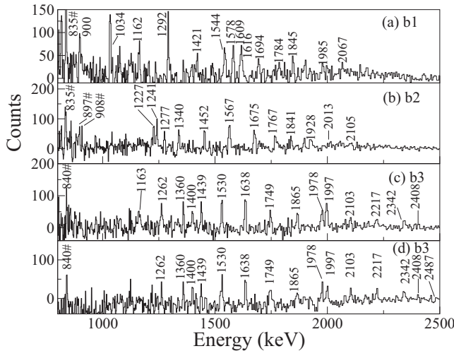
FIG. 2. Summed triple-gated \gamma -ray coincidence spectra of bands b1–b3 in ^{124}\text{Xe} . The spectra in panels (a)–(c) were obtained by using triple gates on all transitions of bands b1, b2, and b3, respectively. The spectrum in panel (d) was produced with a gate on the 1997-keV transition and two gates on all the transitions of b3. Transitions marked by # signs in the various panels stem from low-energy levels which receive the highest-intensity feeding from bands b1–b3.
