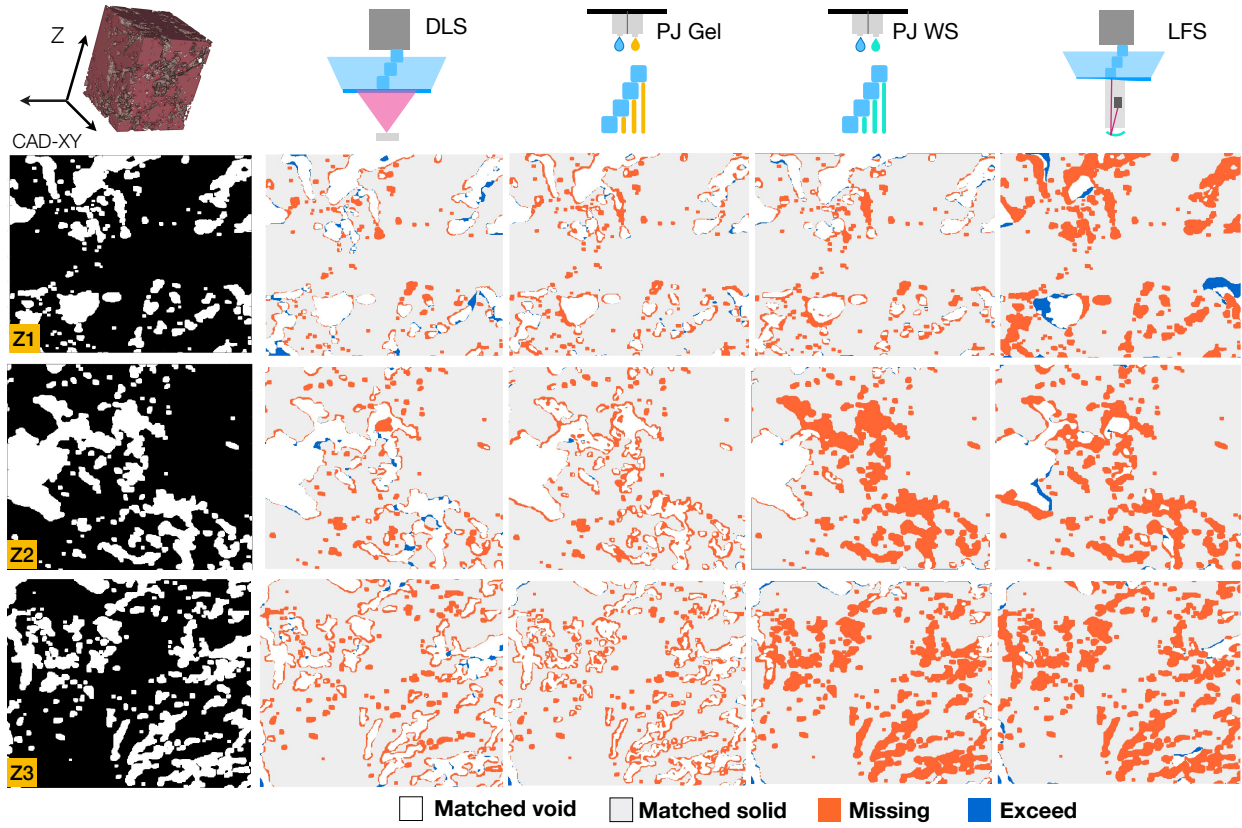
Figure 2: Illustrative cross-sections at different z-depths of matched and mismatched pore geometry for each 3D printing technique tested. Left column shows a 3D rendering of the soil CAD and cross-sections with solid (black) and void (white). Additional columns show the corresponding cross-section produced by the four 3D printing technologies evaluated. The pore space is color-coded (corresponding to the summary of Figure 1) for matched (gray), missing (orange), and excess (blue) volume. All cases lack the smallest void features.
