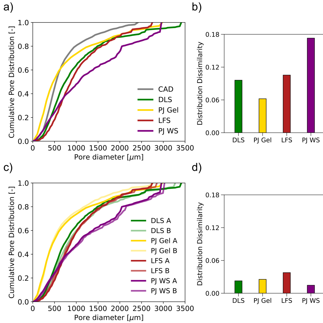
Figure 4: a) Cumulative pore size distribution and b) their corresponding distribution dissimilarity metric for the soil CAD and all printed analogues (accuracy). c) Cumulative pore size distribution and d) their corresponding distribution dissimilarity metric for replicate analogue pairs (repeatability).
