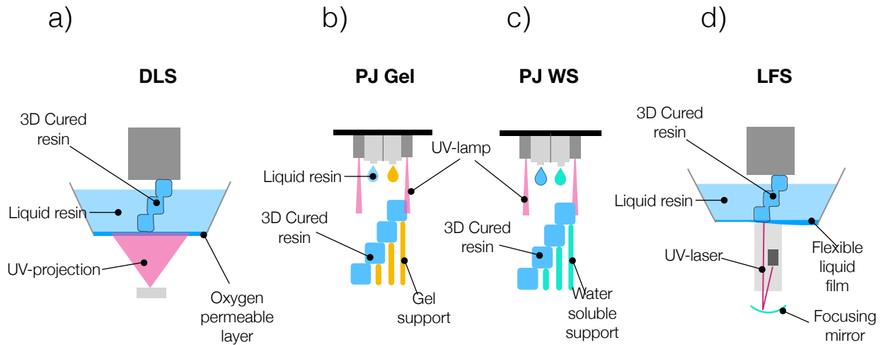
Figure A.5: Schematic of the printing mechanism for the four 3D printers technologies investigated. a) Digital Light Synthesis (DLS). b) UV curing of photopolymers by PolyGet and subsequent removal of the Gel or c) Water support, WS. d) Low Force Stereolithography (LFS).
