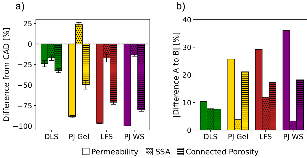
Figure 3: Differences in permeability, specific surface area (SSA), and connected porosity between a) the soil CAD and the printed soil analogues (accuracy) and b) like-printed soil analogues (repeatability).
