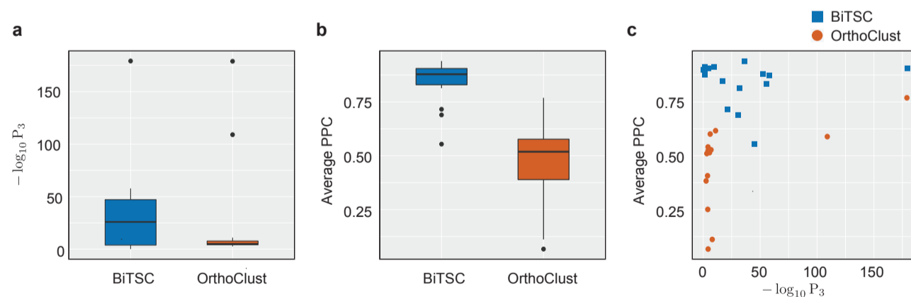
Fig. 3. Comparison of BiTSC and OrthoClust in terms of their identified fly-worm gene co-clusters (Section 3.2.1). (a) Distributions of within-cluster enrichment of ortholog pairs. For BiTSC and OrthoClust, a boxplot is shown for the -\log_{10} P_3 values calculated by the ortholog pair enrichment test (Section S7.3) on the identified gene co-clusters. Larger -\log_{10} P_3 values indicate stronger enrichment. (b): Distributions of within-cluster gene expression similarity. For BiTSC and OrthoClust, a boxplot is shown for the average pairwise Pearson correlation (PPC) between genes of the same species within each identified co-cluster. (c): Within-cluster gene expression similarity vs. ortholog enrichment. Each point corresponds to one co-cluster identified by BiTSC or OrthoClust. The -\log_{10} P_3 and average PPC values are the same as those shown in (a) and (b).
