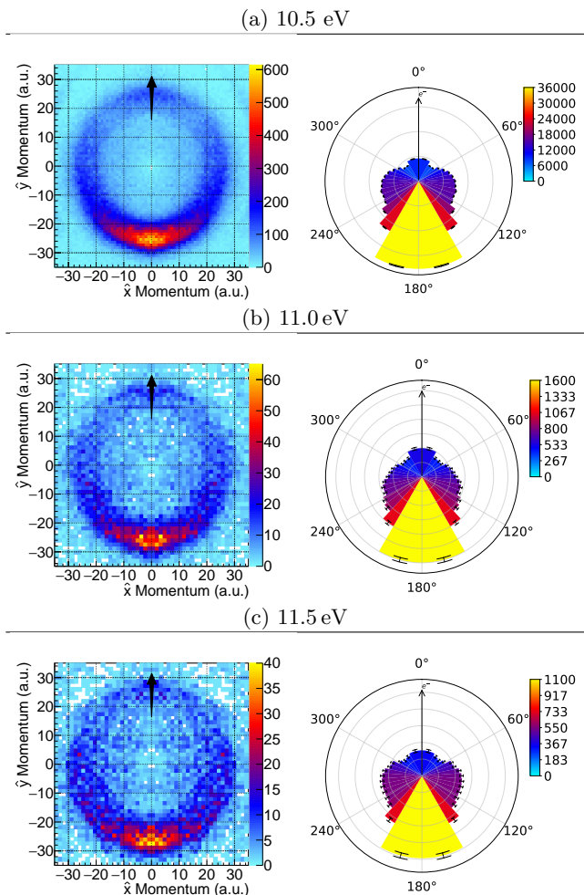
FIG. 5. Left : Momentum images of H^- dissociation from DEA to formamide. Electron is incident in the +y -direction with energy (a) 10.5 eV, (b) 11.0 eV, and (c) 11.5 eV. Right : Histograms of dissociation angle of H^- anions from formamide with incident electron energy of (a) 10.5 eV, (b) 11.0 eV, and (c) 11.5 eV in the direction of 0^\circ . Note: the error bars are purely statistical.
