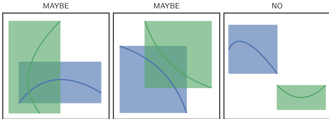
Figure 3.1: Bounding box intersection predicate. This is a cheap way to conclude that two curves don't intersect, though it inherently is susceptible to false positives.
