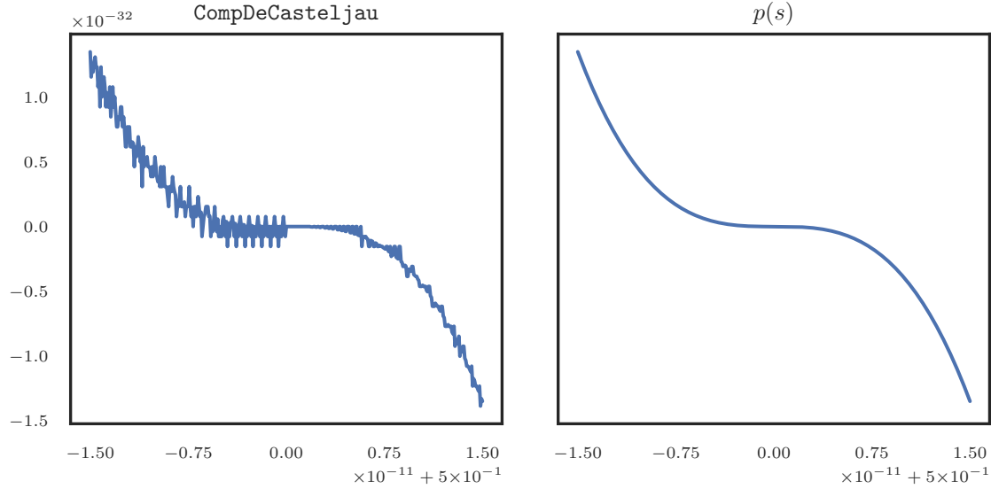
Figure 5.4: The compensated de Casteljau method starts to lose accuracy for p(s) = (2s - 1)^3(s - 1) in the neighborhood of its multiple root 1/2 .
