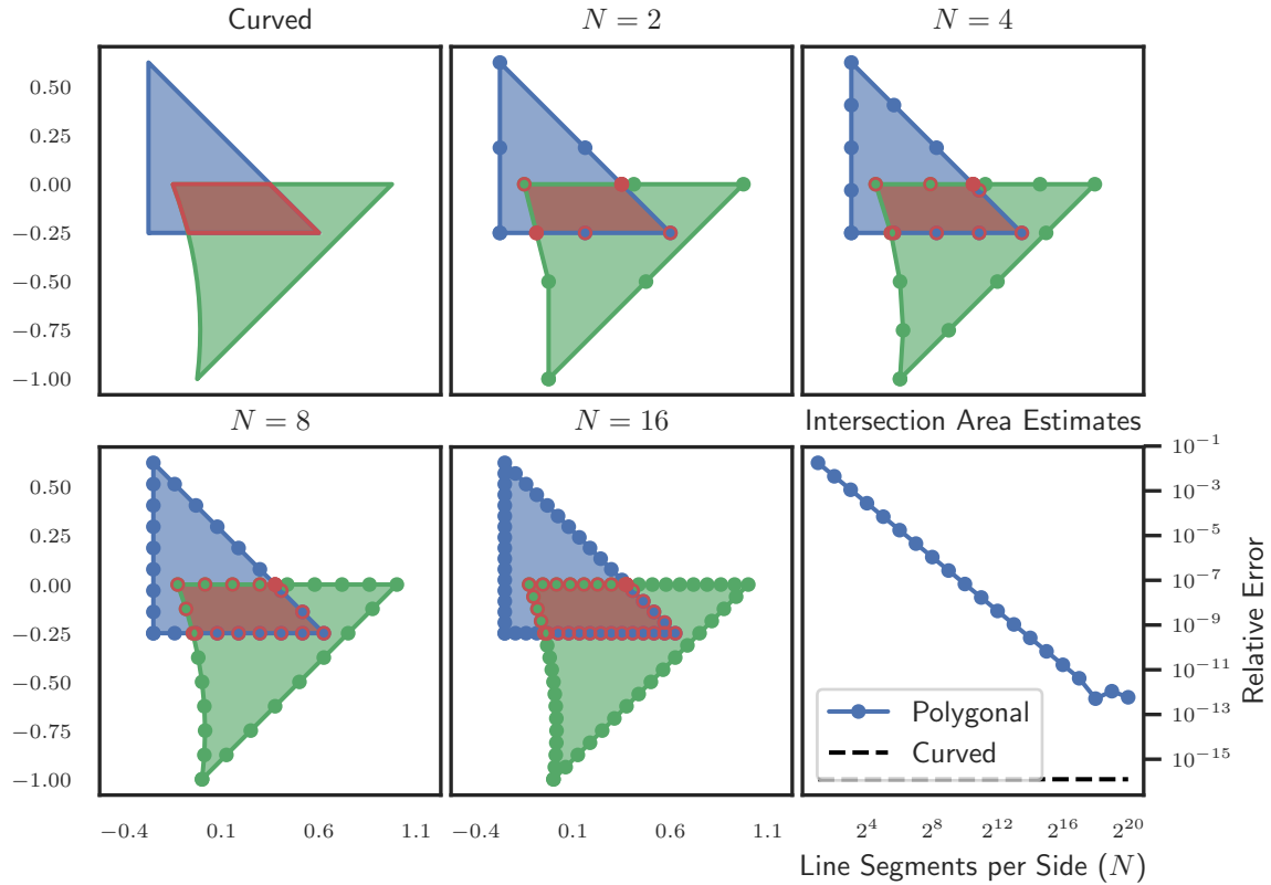
Figure 4.13: Comparing the relative error for the computed area of the intersection of two quadratic Bézier triangles. In one method, the intersection boundary is fully specified as the union of Bézier curve segments and the area is computed correctly to machine precision. In the other, the curved edges are approximated by polygonal paths and the intersection of the resulting polygons is computed.
