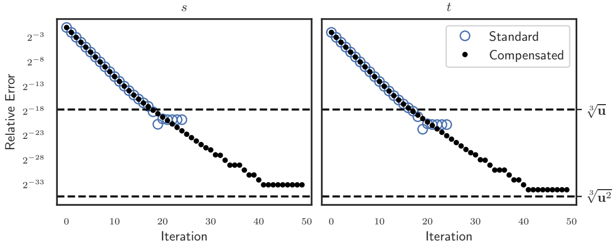
Figure 6.5: Relative error plots for the computed intersection \alpha = \beta = 1/2 when using standard Newton's method and a modified Newton's method that uses a compensated residual.
