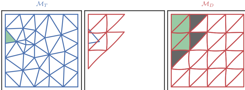
Figure 4.10: All donor elements \mathcal{T}' that cover a target element \mathcal{T} , with an extra layer of neighbors in the donor mesh that do not intersect \mathcal{T} .
