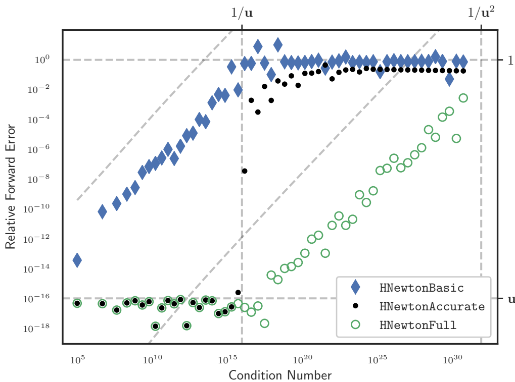
Figure 6.1: Comparing relative error to condition number when using Newton’s method to find a root of p(s) = (s - 1)^n - 2^{-31} , where polynomial evaluation occurs via Horner’s method.
