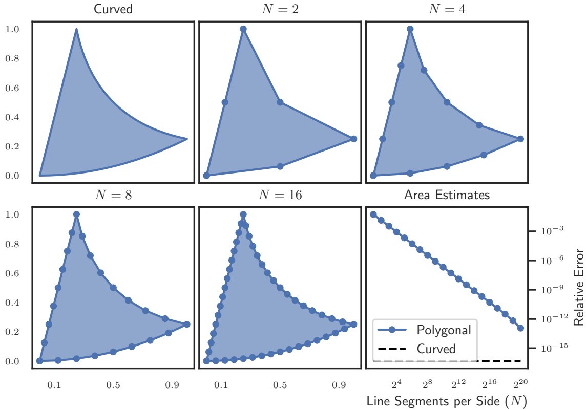
Figure 4.12: Comparing the relative error for the computed area of a quadratic Bézier triangle. In one method, the curved boundary is used and the result is correct to machine precision. In the other, the curved edges are approximated by polygonal paths.
