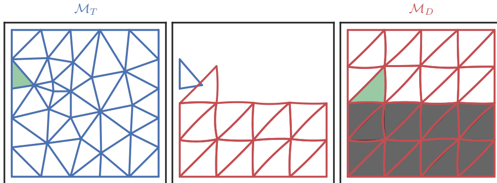
Figure 4.9: Brute force search for a donor element \mathcal{T}' that matches a fixed target element \mathcal{T} .
