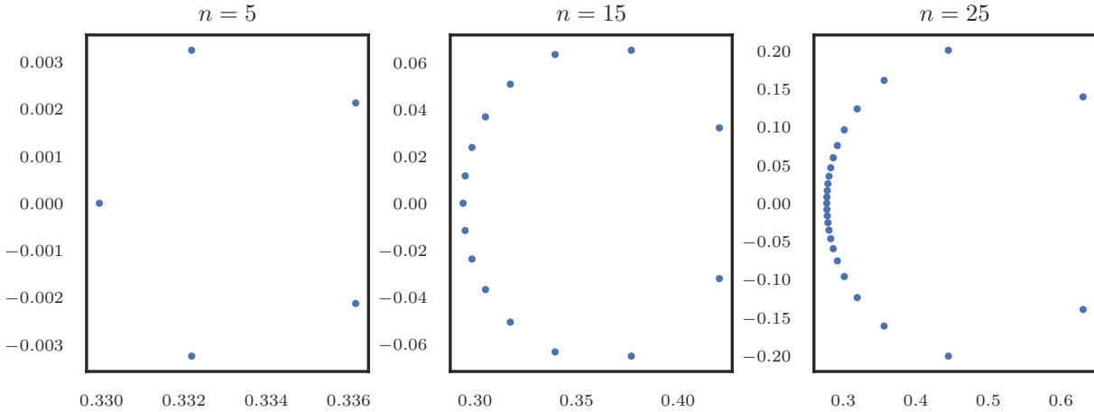
Figure 6.2: Roots of p(s) = (1 - 5s)^n + 2^{30}(1 - 3s)^n for n = 5, 15 and 25 .
