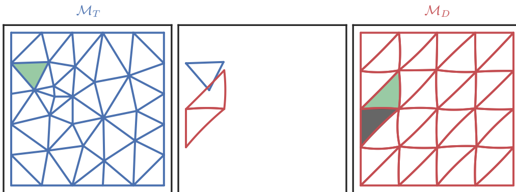
Figure 4.11: First match between a neighbor of the previously considered target element and all the donor elements that match the previously considered target element.
