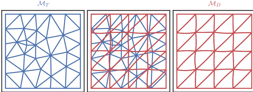
Figure 4.7: Mesh pair: donor mesh \mathcal{M}_D and target mesh \mathcal{M}_T .
