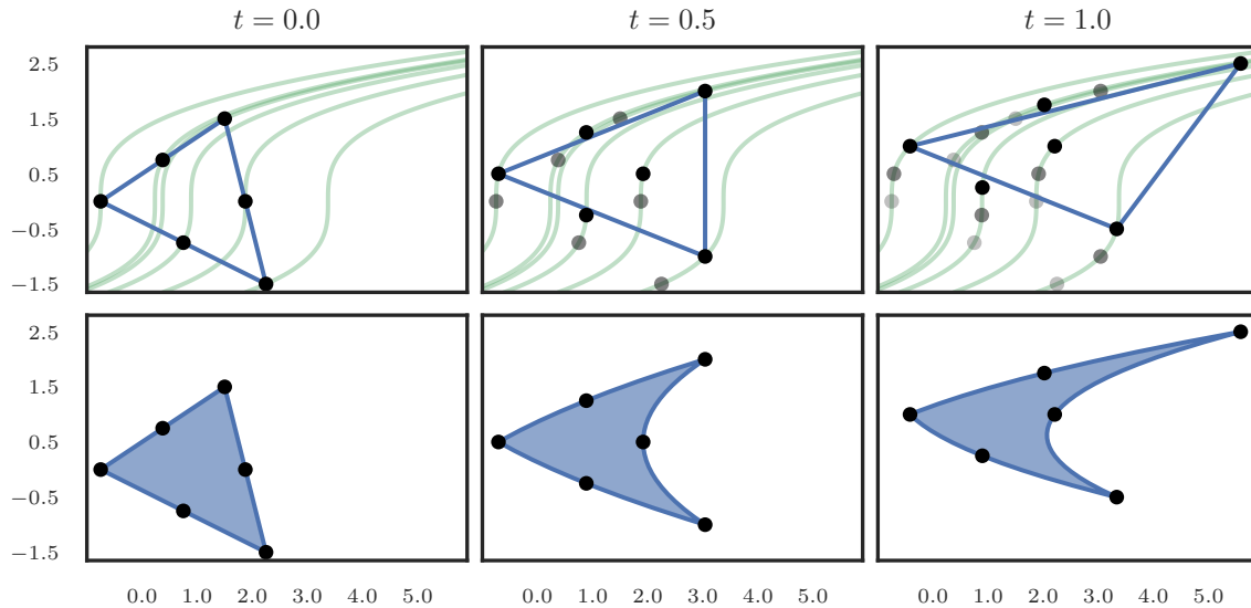
Figure 4.5: Movement of nodes in a quadratic element under distortion caused by particle motion along the velocity field [y^2 \ 1]^T from t = 0 to t = 1 with \Delta t = 1/2 . The green curves represent the characteristics that each node travels along.
