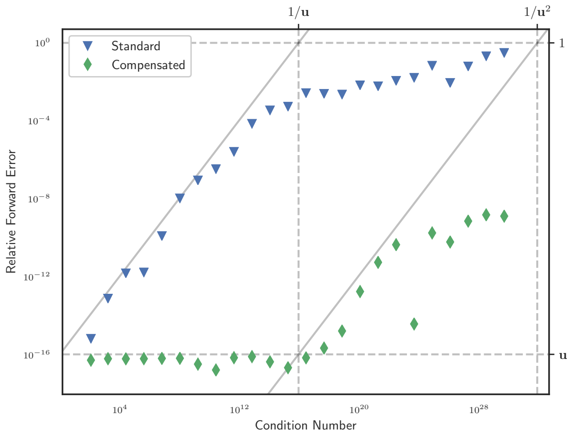
Figure 6.6: Relative error plots for the computed intersection \alpha = \beta = 1/2 when using standard Newton's method and a modified Newton's method that uses a compensated residual.
