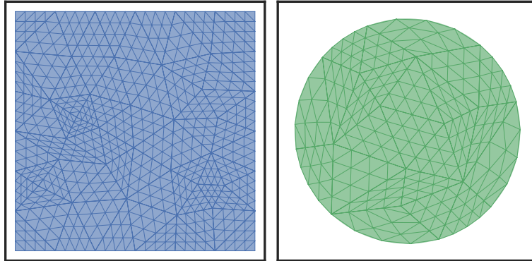
Figure 4.16: Some example meshes used during the numerical experiments; the donor meshes is on the left / blue and the target mesh is on the right / green. These meshes are the cubic approximations of each domain and have been refined twice.
