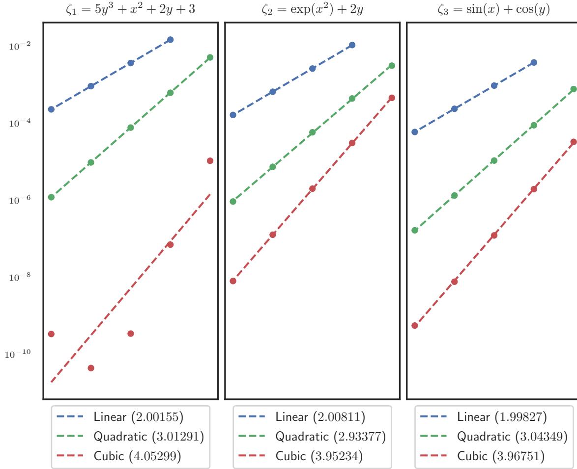
Figure 4.17: Convergence results for scalar fields on three pairs of related meshes: a linear, quadratic and cubic mesh of the same domain.
