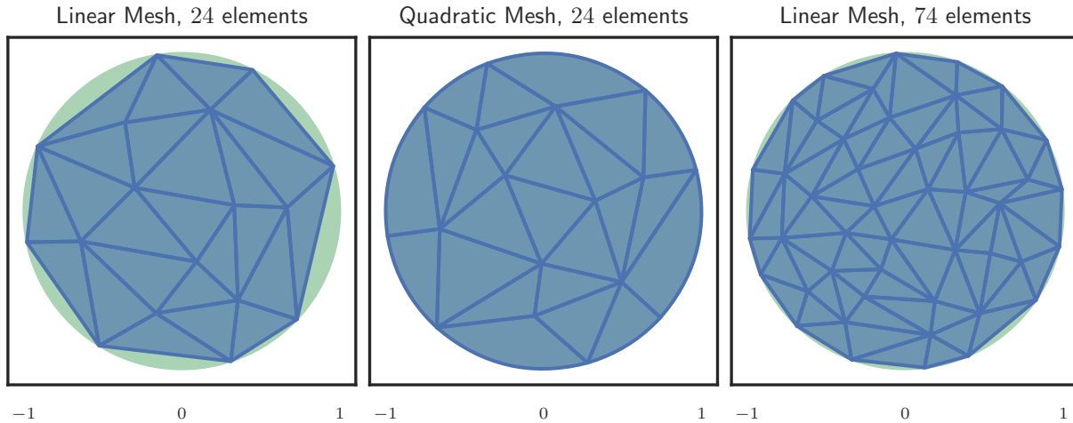
Figure 4.4: Comparing straight sided meshes to a curved mesh when approximating the unit disc in \mathbf{R}^2 .
