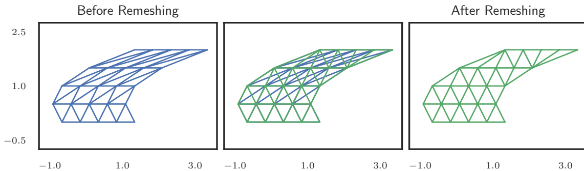
Figure 4.3: Remeshing a domain after distortion caused by particle motion along the velocity field [y^2 \ 1]^T from t = 0 to t = 1 .
