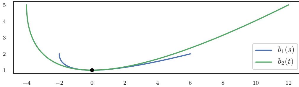
Figure 6.4: Intersection of two Bézier curves that are tangent and have the same curvature at the point of tangency.
