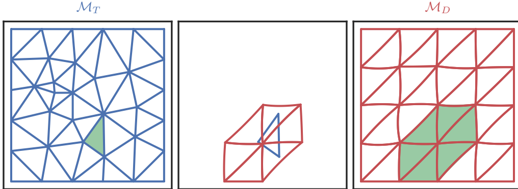
Figure 4.8: All donor elements that cover a target element
