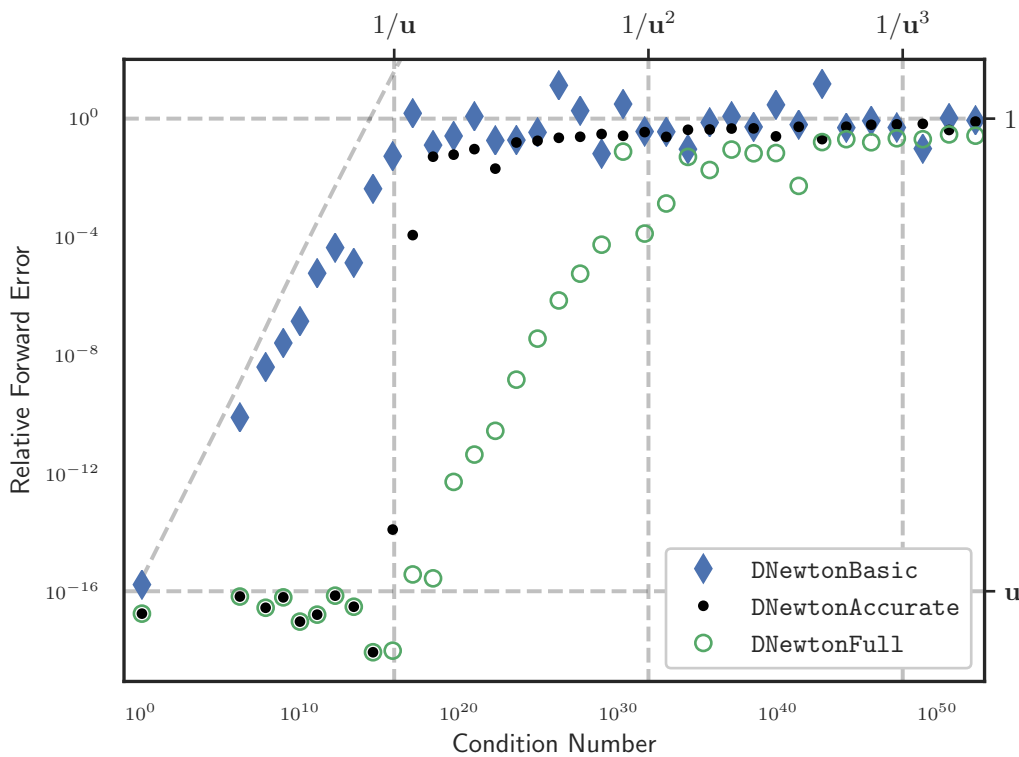
Figure 6.3: Comparing relative error to condition number when using Newton’s method to find a root of p(s) = (1 - 5s)^n + 2^{30}(1 - 3s)^n for n odd.
