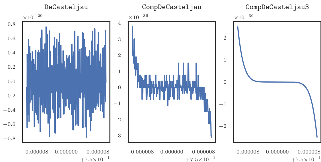
Figure 5.6: Evaluation of p(s) = (s - 1)(s - 3/4)^7 in the neighborhood of its multiple root 3/4 .
