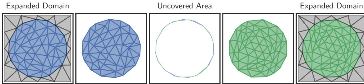
Figure 4.6: Partially overlapping meshes on a near identical domain. Both are linear meshes that approximate the unit disc in \mathbf{R}^2 . The outermost columns show how the domain of each mesh can be expanded so they agree.
