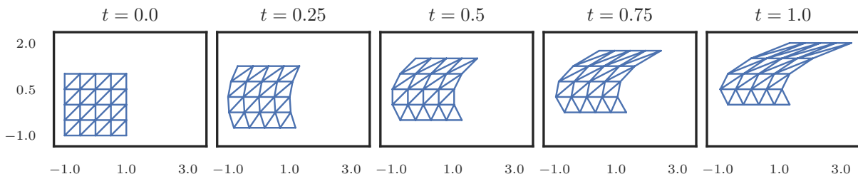
Figure 4.2: Distortion of a regular mesh caused by particle motion along the velocity field [y^2 \ 1]^T from t = 0 to t = 1 with \Delta t = 1/4 .
