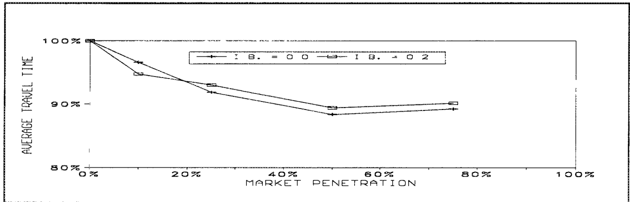
Figure 5. Unequipped Vehicles
