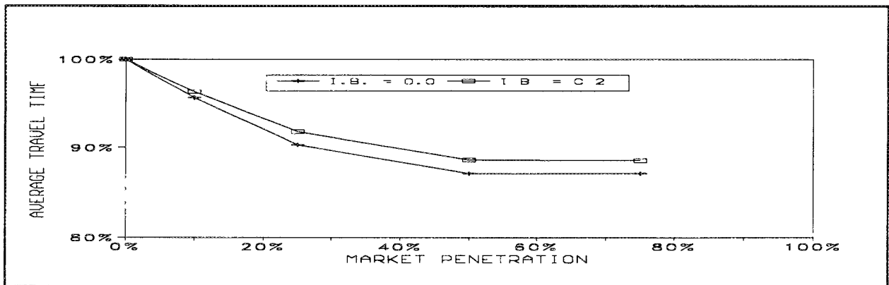
Figure 6. All Vehicles
