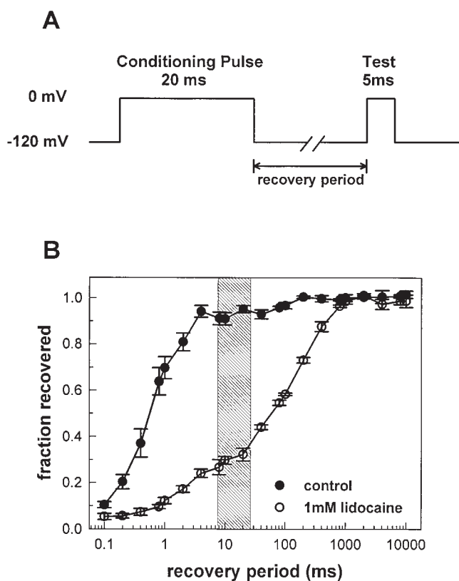
FIGURE 6. Lidocaine slows the repriming of \text{Na}^+ channels after brief depolarizations. A two-pulse recovery protocol was used to assess the rate of repriming of F1304C channels after a 20-ms depolarization to 0 mV. The peak current measured during the test pulse was divided by the peak current measured during the conditioning pulse, and plotted as a function of the recovery period. In the absence of lidocaine, the current recovered almost completely within 10 ms, while in the presence of 1.0 mM lidocaine, the time constant of recovery is roughly 100-fold slower. The shaded area indicates the duration of MTS-ET exposure relative to \text{Na}^+ channel repriming for the protocol shown in Fig. 7 A.
