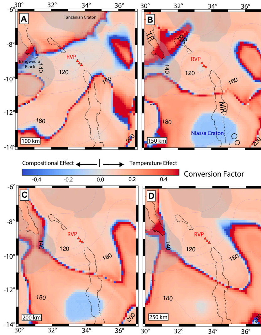
FIGURE 8 Lateral distribution of the conversion factor between the S-wave velocity perturbations ( dlnVs ) and our final density anomalies at (A) 100 km, (B) 150 km, (C) 200 km and (D) 250 km depth. Black circles in Figure 8B represent the location of Ring-Complexes observed on Shuttle Radar Topography Mission (SRTM) Digital Elevation Model (DEM) by Njinju et al. (2019a).
