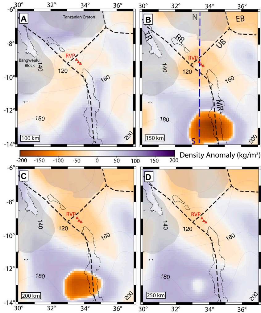
FIGURE 4 Depth slices showing in situ density anomalies beneath the RVP and surroundings at (A) 100 km, (B) 150 km, (C) 200 km and (D) 250 km depth. Red triangles represent the Rungwe Volcanic Province (RVP). Black lines indicate the outline of rift lakes. Blue contours show lines of equal lithospheric thickness at 20 km intervals from Fishwick (2010). Black dotted lines delineate plate boundaries from Stamps et al. (2008). Blue profile N-S in Figure 4B is the profile location for Figure 5B.
