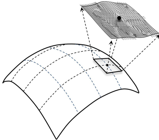
Figure 1. The schematic of the extended harmonic map (EHM) theory. The EHM can be understood as a local potential field added to the conventional harmonic map (HM). This addition changes the local space curvature and generates anisotropic/asymmetric space-time, which can be described as a special case of Finsler surface.
