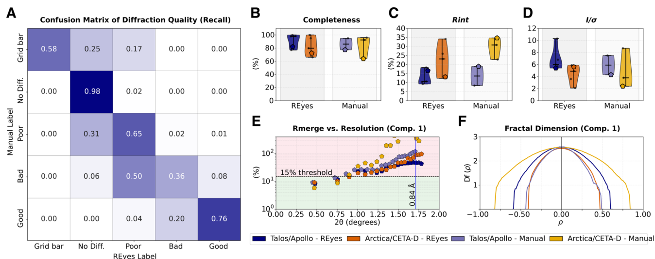
Figure 7. Comparison of diffraction data quality metrics obtained by REyes. (A) Row-normalized (recall) confusion matrix showing how each manually assigned category (rows) maps to REyes classifications (columns). (B–D) Violin plots comparing (B) completeness, (C) R int, and (D) I /σ of solutions from single microED movies obtained by REyes and acquired manually. Pentagon point represents (S,S)-salen ligand 1 . (E) R merge values plotted against 2θ resolution. (F) Fractal dimension measurements for REyes versus manual data collection.
