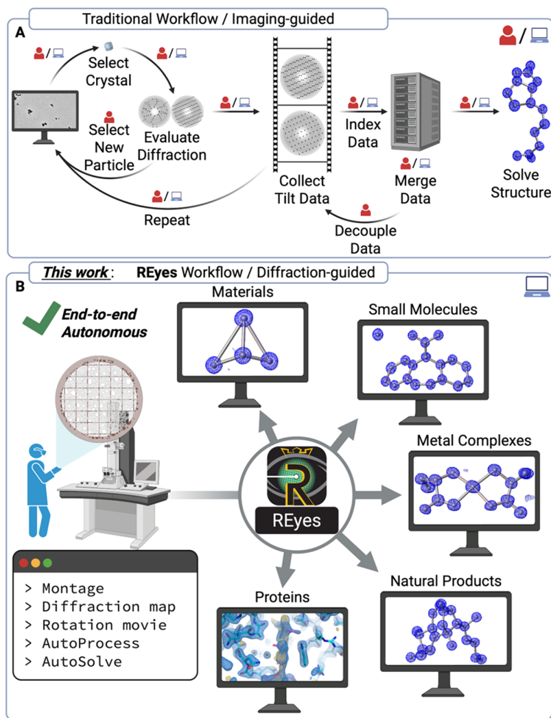
Figure 1. Traditional and fully autonomous microED workflows. (A) Traditional workflow using imaging mode and expert data curation. (B) Autonomous workflow using REyes, incorporating a diffraction atlas for spatially aware sample-independent data acquisition and automated indexing and phasing for preliminary structural solutions.
