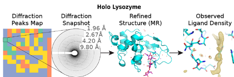
Figure 6. REyes, AutoProcess, molecular replacement, and refinement results of an automated microED acquisition of tetragonal holo-lysozyme. REyes “Quality” diffraction map of a grid square led to a single-movie solution, diffraction snapshot at 2.0 Å max resolution of the target selected by REyes using the Arctica/Apollo system, refined structure of lysozyme phased using molecular replacement, gold-mesh represents 3\sigma NAG 3 ligand in the F_o - F_c map.
