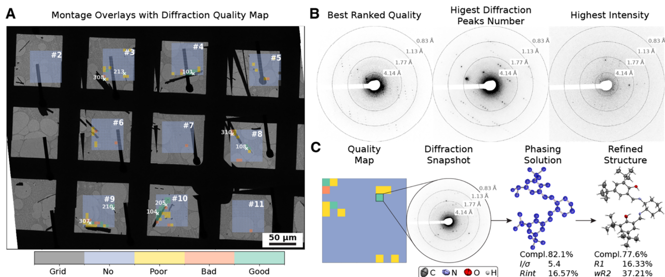
Figure 3. REyes, AutoProcess, and AutoSolve outcomes for a sample. (A) Diffraction quality map of the (S,S)-salen ligand 1 grid. (B) Diffraction snapshots of the highest-ranked targets by quality, peak number, and intensity. (C) Target 213: REyes ‘Quality’ diffraction map of a grid square led to a single-movie solution, diffraction snapshot at 0.8 Å max resolution of the target selected by REyes, Fobs map for ab initio preliminary solution at 0.8 Å, and refined structure of salen ligand 1 . Priority targets included items 101, 205, and 307 (Table 1).
