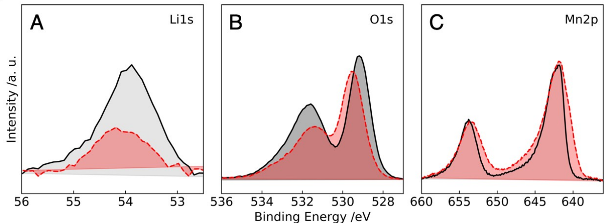
Figure 4. A) Li 1s, B) O 1s and C) Mn 2p XPS spectra of the as-received (in black) and acid treated (in red) LR-NMC oxide powders.
