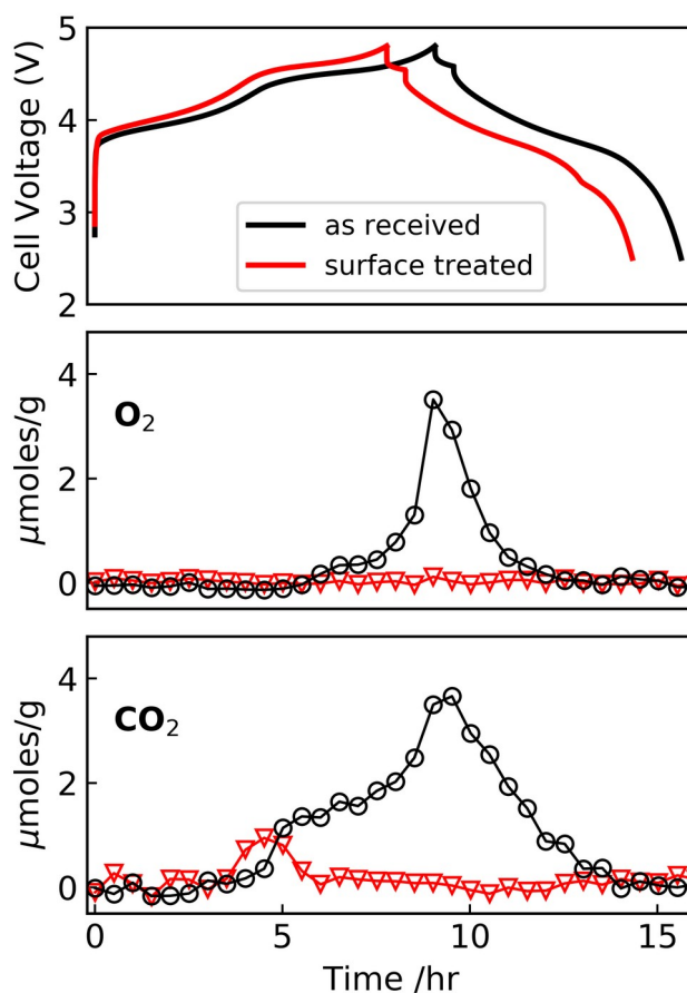
Figure 1. The first cycle charge-discharge profile (top) of the as-received (in black) and surface-treated (in red) LR-NMC cathodes with accompanying \text{O}_2 and \text{CO}_2 evolution as measured by DEMS (rate= 0.1 \text{Li}^+ /hour).
