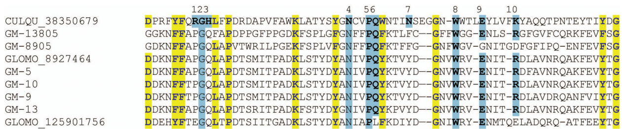
Figure 2 Alignment of the active center region of Culex quinquefasciatus endonuclease with Glossina morsitans morsitans proteins of the same family. The ten amino acids making contact to substrate, based on the Serratia marcescens crystal structure, are shown in turquoise background for the Culex and Glossina sequences. Note the absence of three conserved residues in the tsetse proteins. Other conserved residues are marked in yellow background.
