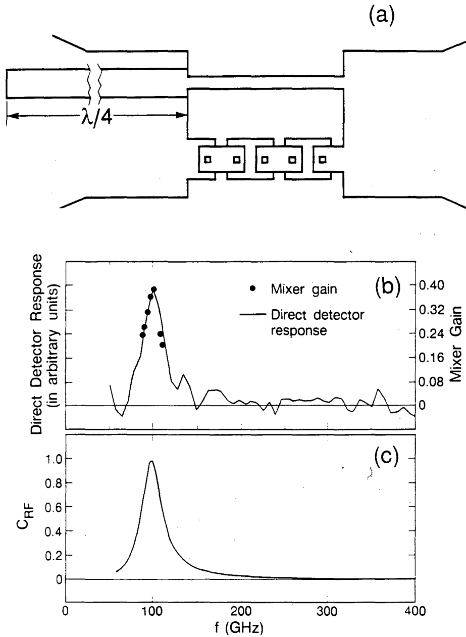
Fig. 6.10 a) Diagram of an 5-junction array of SIS junctions with an inductive wire as a tuning element. The wire is RF-shorted by a \lambda/4 section of microstrip transmission line. b) Measured frequency response of the structure shown in a). c) Computed RF coupling coefficient of the structure shown in a).
