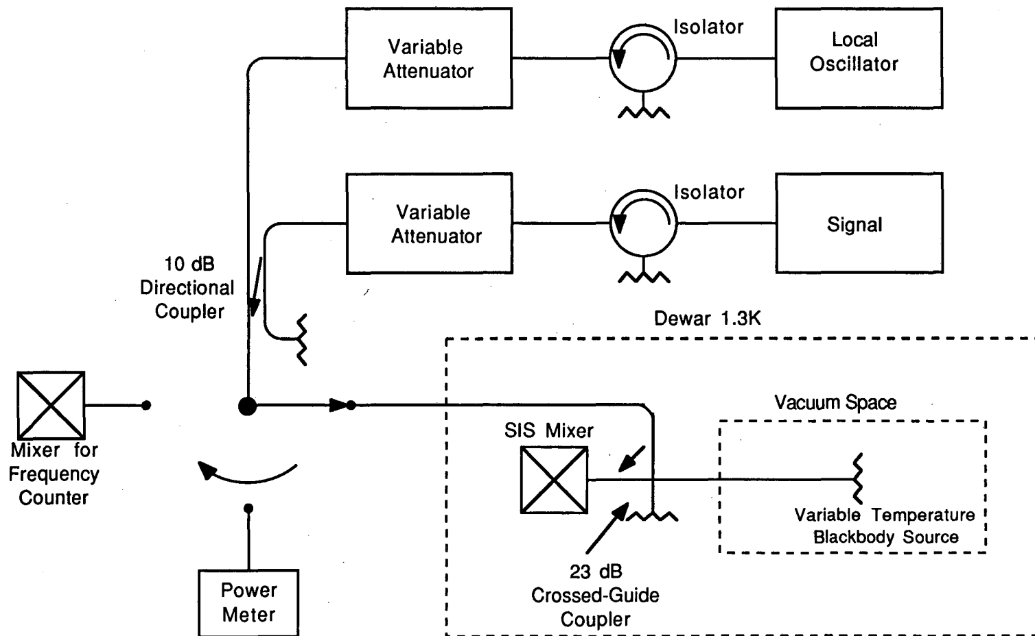
Fig. 5.1 Block Diagram of RF Measurement Apparatus
