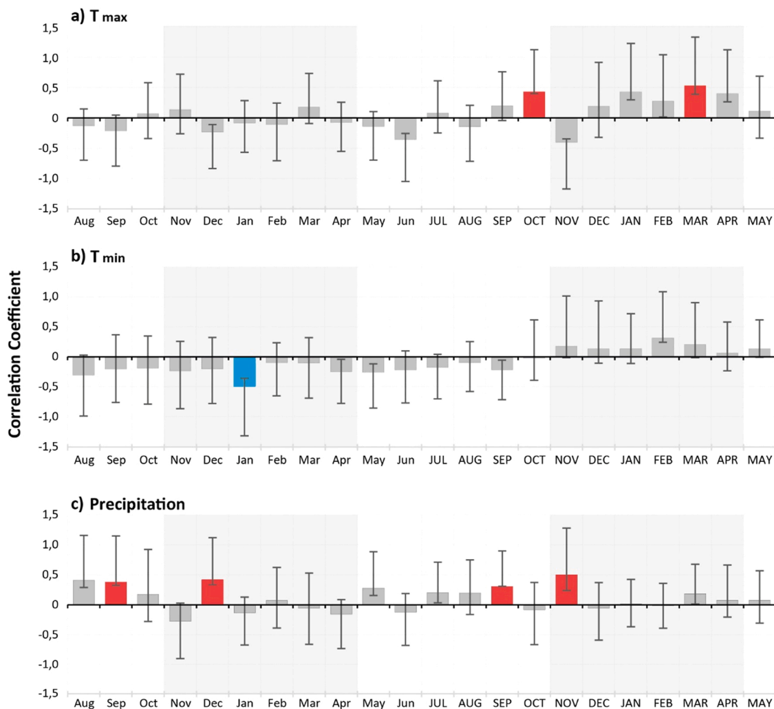
Fig. 5. Correlation coefficient between TRW and a) T_{\max} , b) T_{\min} and c) precipitation. The gray shaded areas represent the growing seasons from November to April. Significant correlation coefficients ( \rho < 0.05 ) are indicated by red (positive) and blue (negative) colored columns.
