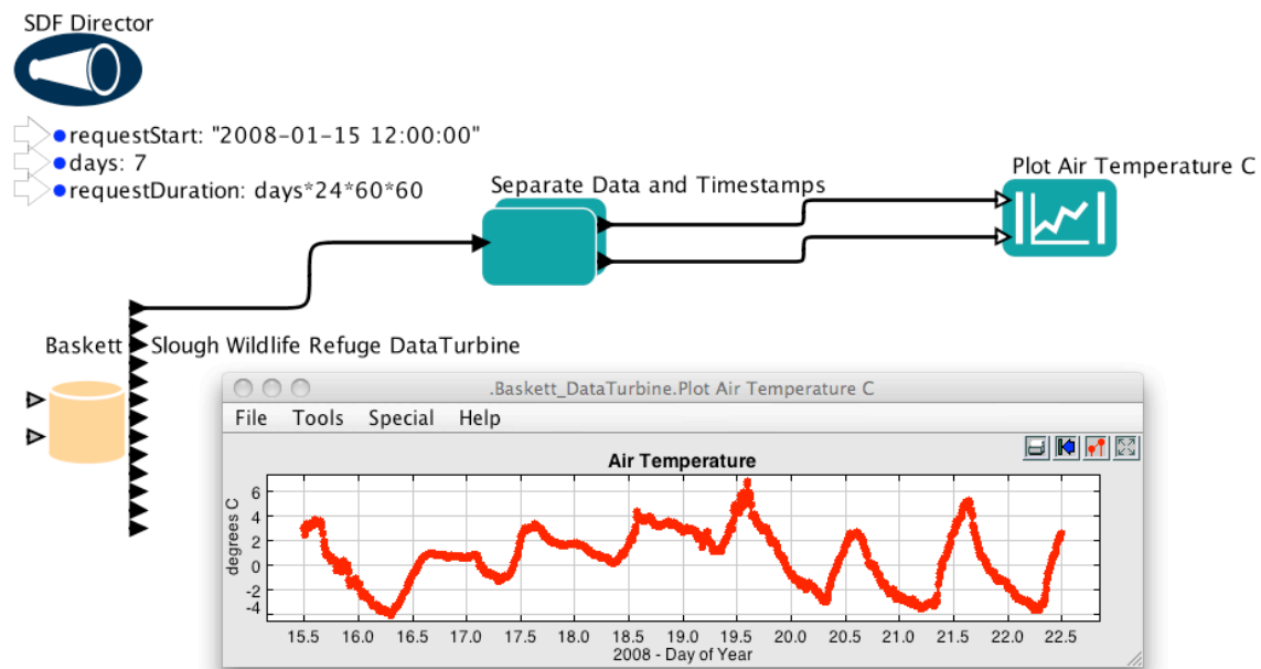
Figure 2. An exploratory analysis workflow that plots sensor data from a DataTurbine server. There are three actors: a DataTurbine data source actor (with 13 output ports), a composite actor that separates a DataTurbine channel into its Data and Timestamp components, and a plotting actor that plots the timeseries. Three relations (“links” along which tokens flow) connect the actors. The Synchronous Dataflow (SDF) director controls execution of the workflow. For convenience, three parameters positioned beneath the director allow for easily changing the time-range of data that the DataTurbine actor will output during execution. The resultant interactive plot is also shown.
