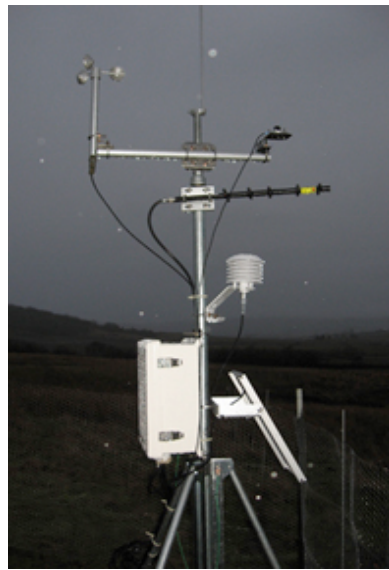
Figure 1. Meteorological station for the terrestrial ecology use case. From left to right, starting at top: anemometer, lightning rod, quantum point sensor, directional antenna, relative humidity and temperature sensor within gill radiation shield, enclosure and solar panel.
