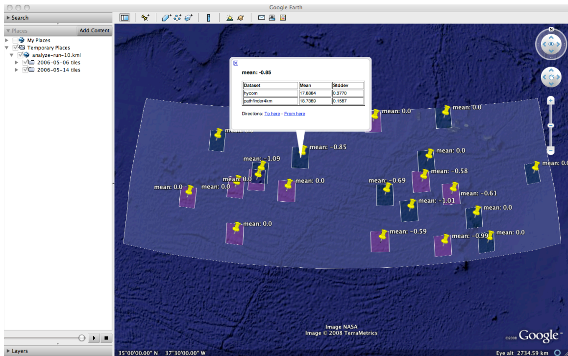
Figure 7. The result of an execution of the workflows in Figures 5 and 6 is shown above, displayed in Google Earth. Specific points display the difference in mean temperatures between two datasets.
