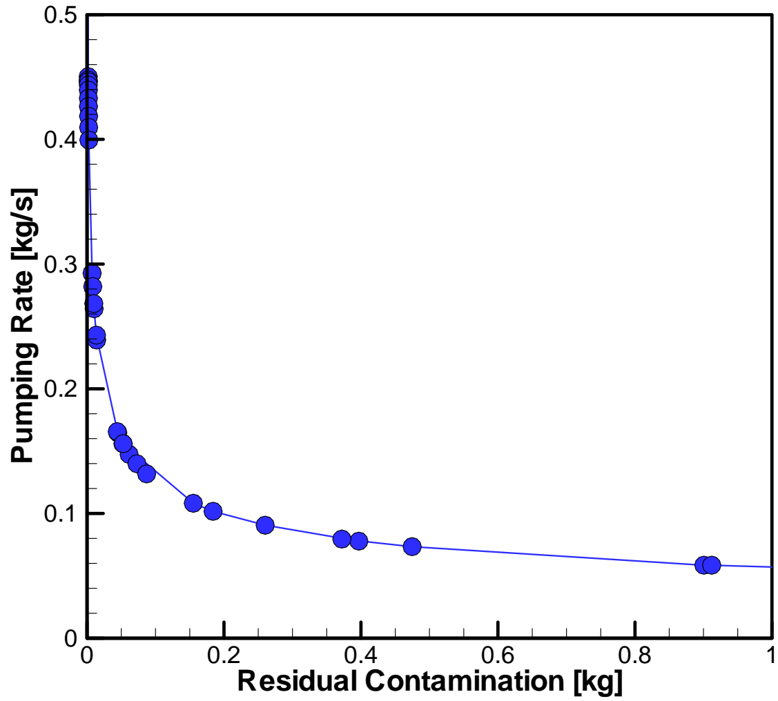
Figure 37. Pareto frontier.
