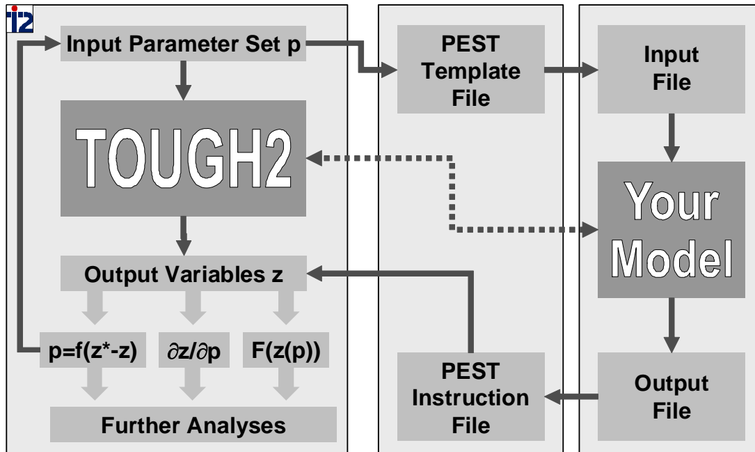
Figure 1. iTOUGH2-PEST architecture.
