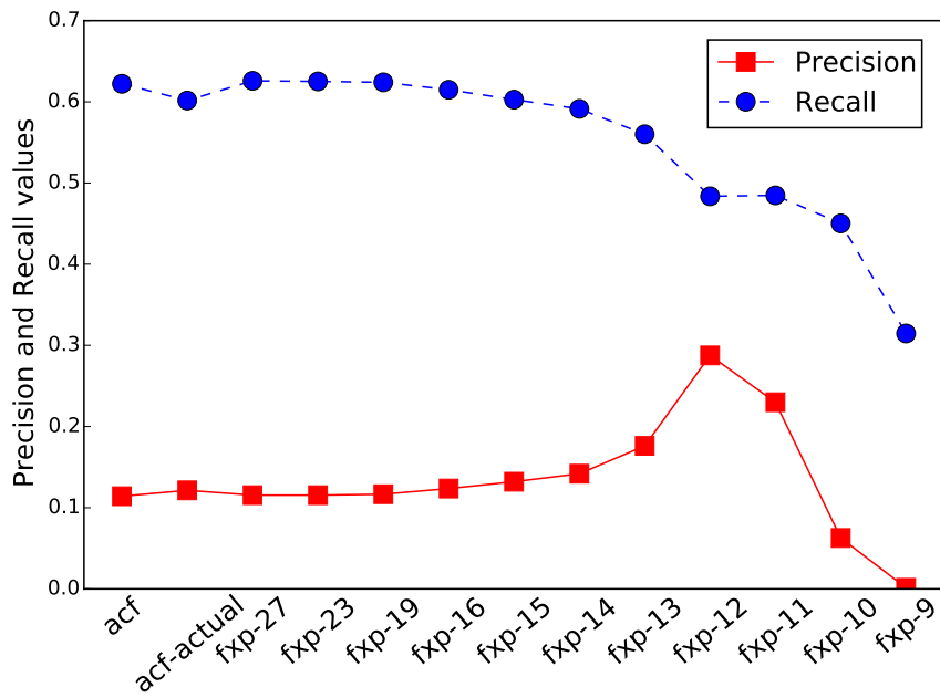
Figure 4.10: ACF fixed-point detection results for Caltech Benchmark.
