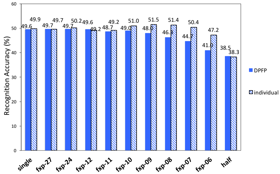
Figure 5.11: UCF50 dataset recognition results using DBFP and individually trained centers.
