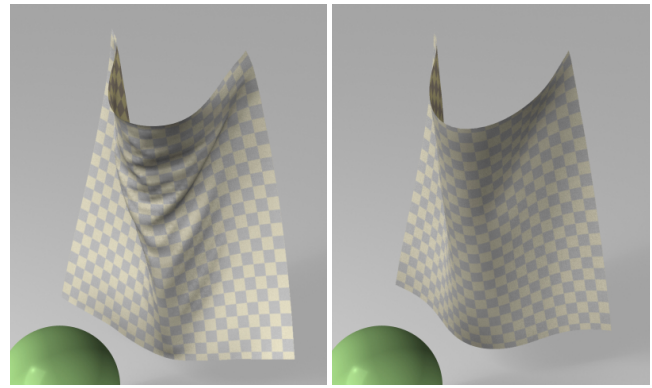
Figure 7: A pair of cloth sheets showing the effect of bending limits on wrinkle formation. Loose bending angle limits [-60^{\circ}/\text{cm}, 60^{\circ}/\text{cm}] (left) allow small wrinkles, while tighter limits [-30^{\circ}/\text{cm}, 30^{\circ}/\text{cm}] (right) prevent small wrinkles from forming.
