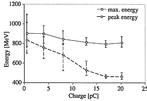
Fig. 10. The peak energy and maximum energy versus charge for 33 mm long, 300 \mu\text{m} diameter capillary. Out of a set of 51 shots, 37 shots were observed with electrons above 400 MeV. Bars show minimum and maximum shots.
