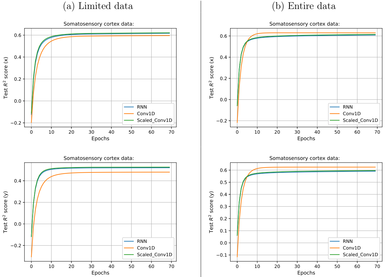
Figure 5.5: R^2 score for the two dimensional reaching task described in section 5.5 . The data is recorded from the primary somatosensory cortex of macaques. (a) Limited data: The models are trained on 4.5 minutes of recorded data. (b) Entire data: the whole recording ( \approx 51 mins) is used to compare the performances. For both cases we used mini-batch (batch size = 128) gradient descent with lr = 10^{-4} .
