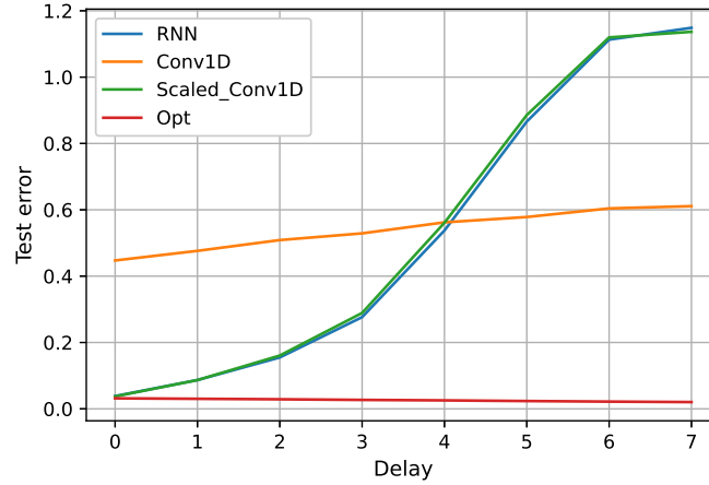
Figure 5.3: Test performance with respect to delay. For this task we have n_h = 1000 , N_{\text{tr}} = N_{\text{ts}} = 10 , n_x = 15 , n_y = 1 , and T = 20 . The delay is added manually by shifting i.e. \mathbf{y}_t = \mathbf{x}_{t-\text{delay}} and the output SNR = 20 dB.
