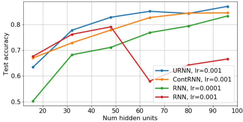
Figure 4.4: Accuracy on Permuted MNIST task for various models trained with RMSProp, validation-based early termination, and initial learning rate 1e-3 . (1) URNN model: RNN model with unitary constraint; (2) ContrRNN: RNN with a contractivity constraint; (3 & 4) RNN model with no contractivity or unitary constraint (two learning rates). We see contractivity improves performance, and unitary constraints improve performance further.
