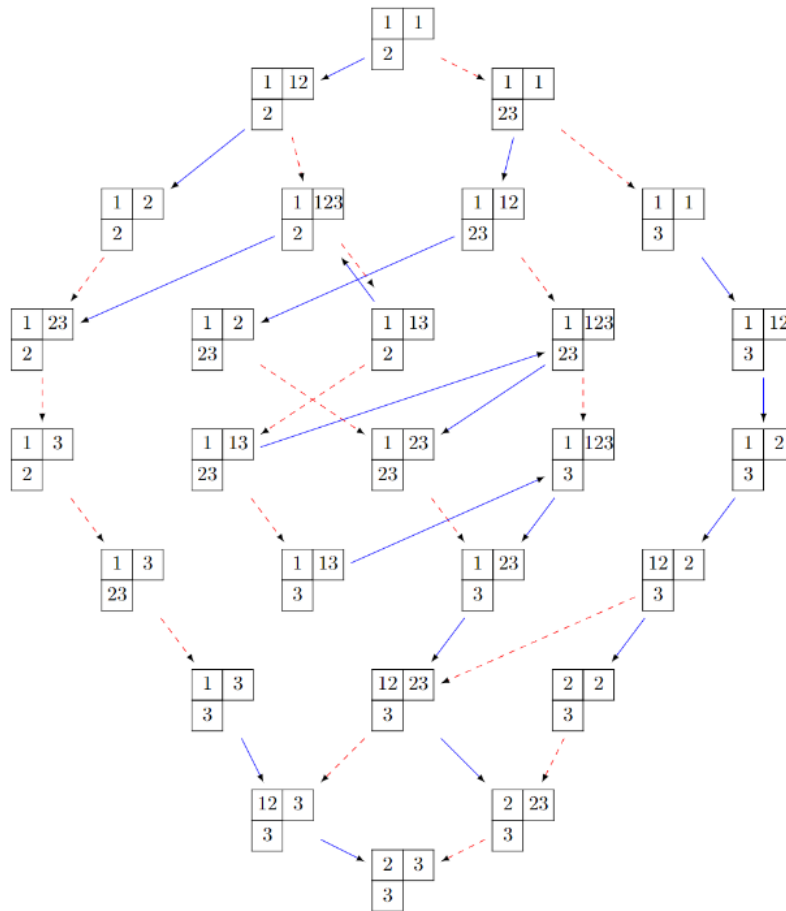
Figure 4.1: The 27 elements of \mathcal{B}_3 with shape (2, 1) .
