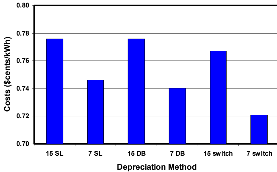
Figure 8. The cost of power generation (only capital and fixed O&M costs, excluding fuel and variable O&M costs) under different depreciation methods and schedules, expressed per kWh of power produced in a 100 MWe cogeneration system.
