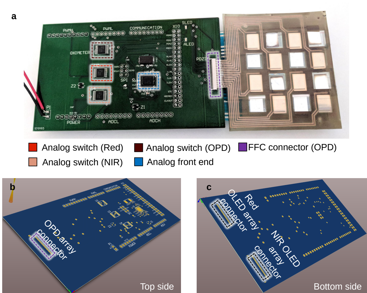
Figure 5.12. Control electronics and connections of the oximeter system. (a) The red and NIR OLED arrays and the OPD array are connected to the control electronics using FFC connectors. These connections then go through three analog switches to the analog front end (AFE 4490). The AFE connects to an Arduino Due microcontroller over Serial Peripheral Interface (SPI) bus, which provides software control of the oximeter array. (b) The top side of the control board, which shows the OPD array connector. (c) The bottom side of the control board, which shows the red and NIR OLED array connectors.
