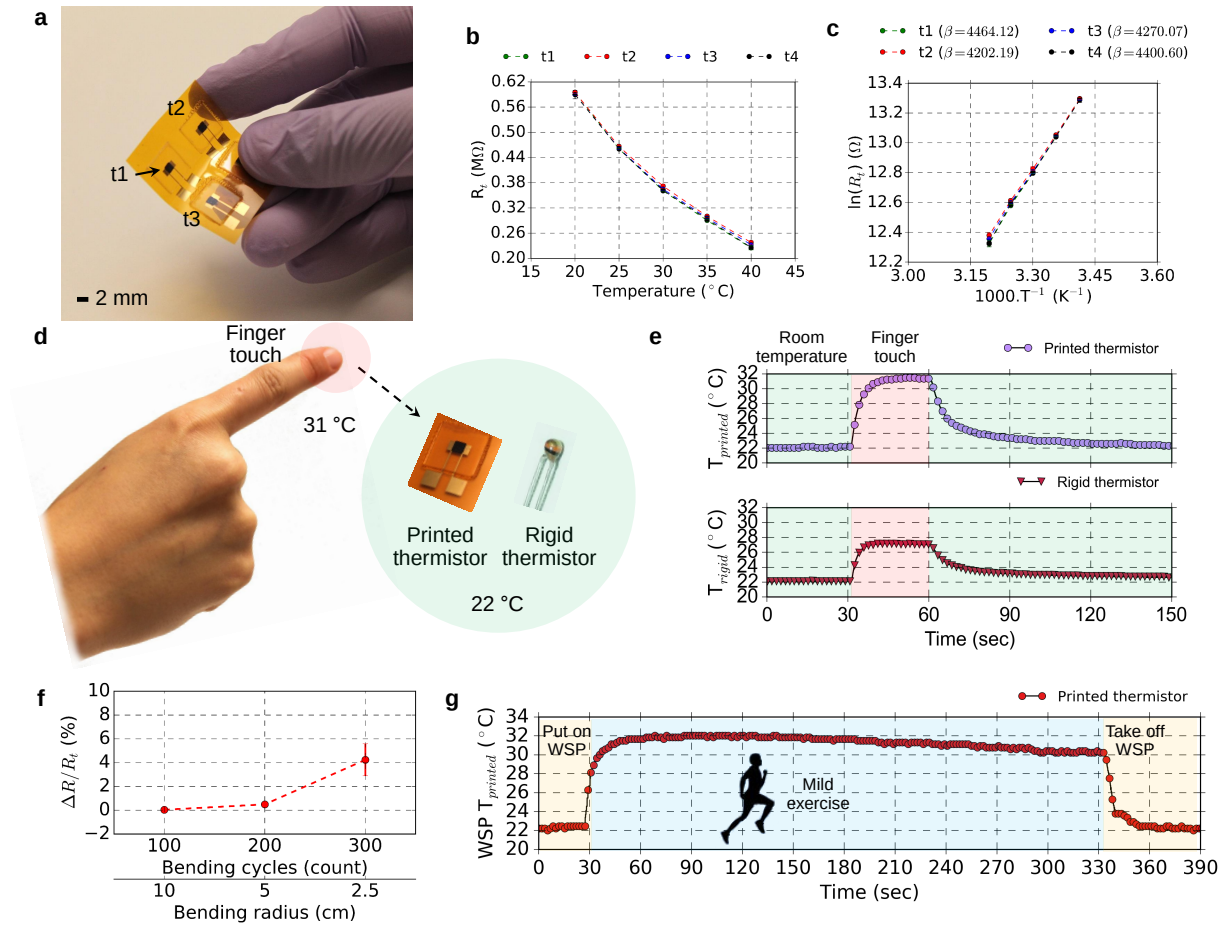
Figure 6.5. Characterization and dynamic testing of the stencil-printed thermistors. (a) Photograph of stencil-printed thermistors composed of NiO nanoparticles and PSBR binder on Kapton ® PI substrate. The four thermistors are labeled t1, t2, t3, and t4. (b) Resistance vs. temperature plot for the thermistors. (c) \beta plot of the printed thermistors. (d) Characterization of the dynamic response of the printed thermistor. The printed thermistor and a commercial rigid thermistor are used to study the dynamic response. Both thermistors are touched with an index finger to record the change in temperature (22 to 31 ^{\circ}C ). (e) The top panel shows the temperature read by the flexible thermistor and the bottom panel shows the temperature read by the rigid device. At normal condition (green), both thermistors show 22 ^{\circ}C , after touching the thermistors (red), the resistance drops due to the rise in temperature. As a result, the printed thermistor show 31 ^{\circ}C , and the rigid thermistor show 27 ^{\circ}C . (f) Durability testing of the printed thermistors. Bending radii of 10, 5, and 2.5 cm are used, and the thermistors are subjected to 100 bending cycles at every bending radius. The room temperature resistance of the thermistors roughly changed by 0, 0.5, and 4%, respectively (the error bars represent data collected from 8 devices). (g) Real-time temperature monitoring using the thermistor. The thermistor accurately measured skin temperature of 30 - 32 ^{\circ}C during the exercise (blue overlay).
