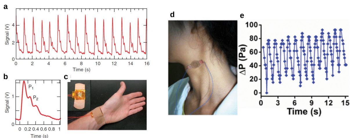
Figure 1.6. HR monitoring using pressure sensors. (a-c) Pulse wave of the radial artery measured with a pressure sensitive polymer transistor. (a) Real-time transient pulse signal. (b) Averaged signal from 16 periods (separate measurements). (c) Photo showing the placement of the sensor on the radial artery of a person. Reprinted by permission from Macmillan Publishers Ltd: Nature Communications [42], copyright (2013). (d,e) Monitoring pulse and blood pressure variation using a droplet-based pressure sensor. (d) The pressure sensor is applied on the skin surface above the carotid artery. (e) Blood pressure variations, as well as the pulse signal, are observed. Reproduced with permission [43]. Copyright 2012, Royal Society of Chemistry.
