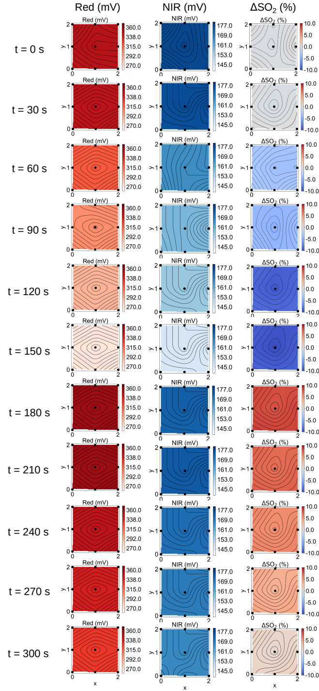
Figure 5.19. 2D contours maps of the red and NIR channels, and change in oxygen saturation ( \Delta SO_2 ) at every 30 s interval for the in-vivo oxygen saturation monitoring test with the ROA as shown in Fig. 5.17.
