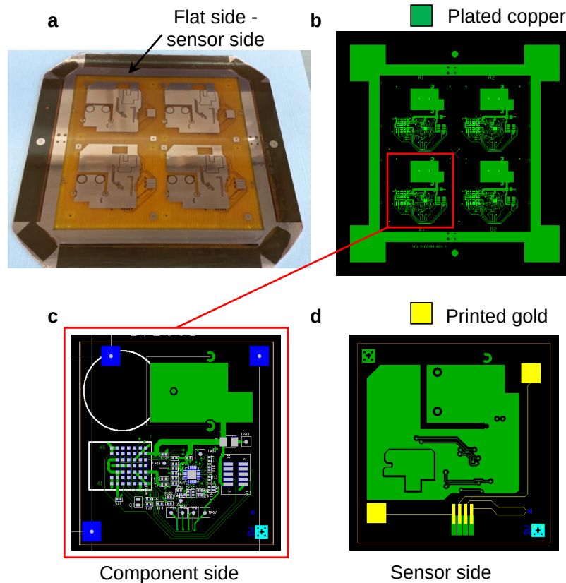
Figure 6.8. Fabrication frame and layout of the WSP. (a) A Kapton® PI substrate is mounted on a 1.27 mm thick frame. Each frame contains four WSPs. The flat side of the frame where sensors are printed, is displayed. (b) The layout of the full panel consisting of four WSPs. Green patterns represent the plated copper. (c) The layout of the component side. (d) The layout of the sensor side: green represents plated copper while yellow represents the printed gold. Alignment marks are visible, which are used to align the gold layer to the copper layer.
