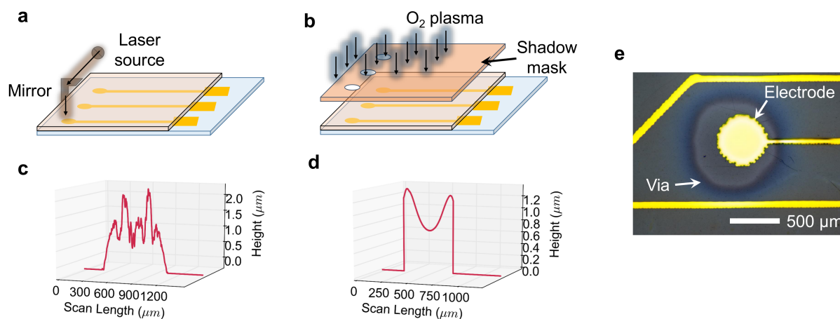
Figure 2.3. Methods for removing the dielectric layer (Cytop) from the electrodes. (a) Laser drilling to open via through the dielectric layer. (b) O 2 plasma etching using a shadow mask to selectively etch the dielectric layer. The surface profile of an electrode after (c) laser drilling and (d) plasma etching. (e) Micrograph of an electrode after plasma etching - etched area encircled by a dark Cytop layer, which is clearly visible; also the exposed electrode is shown.
