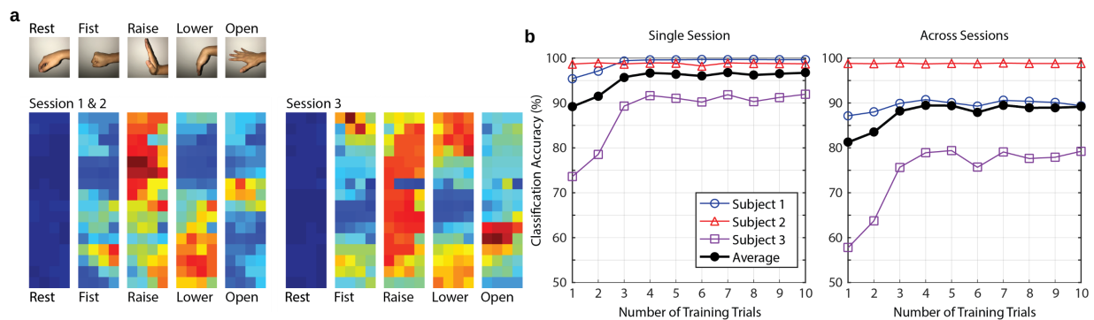
Figure 2.23. Results from the flexible EMG recording system. (a) Dataset gestures with the associated normalized activity maps for different sessions (Subject 1 shown). Pixels correspond to electrode positions in the array. (b) Classification accuracy for different number of training trials.
