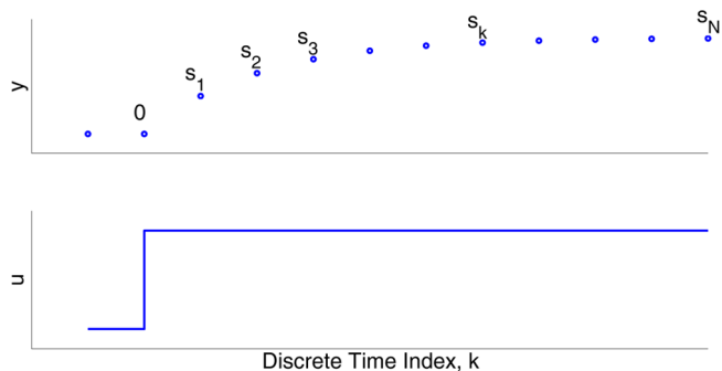
Figure 5. Finite step response model.
