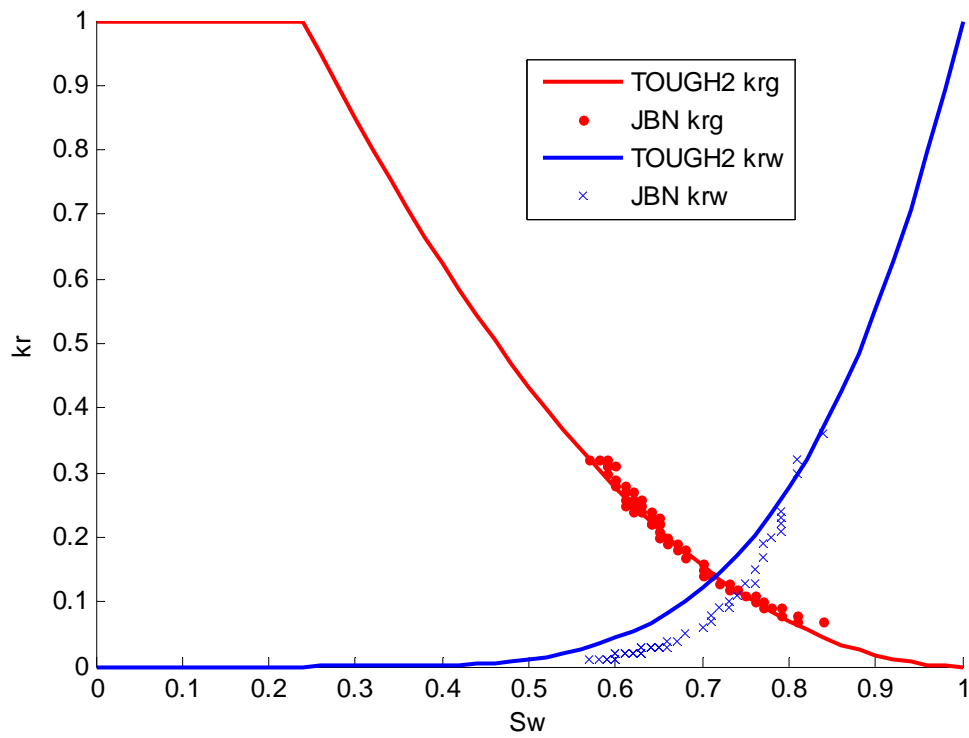
Figure 7 – Comparison between Brooks-Corey curves and JBN method for Nitrogen during primary drainage.
