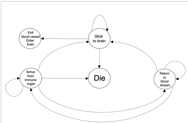
FIGURE 2 | Representative dynamics of the scenarios encountered by an immune cell while coming to the ischemic brain in response to chemokines and DAMPs. The Die and the Exit blood vessel, Enter brain states refer to what would take place at the blood vessels and the brain, respectively. Within a computational framework, the two aforementioned states would be referred to as absorbing states because once an immune cell enters either of those conditions it will not leave that state. Each transition can be associated to a transition probability with the system approximated by a Markov chain. It would be expected that the state transition probabilities will be time-varying and also dependent on a common set of biological variables.
