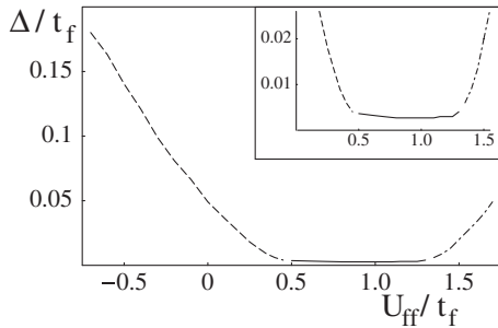
FIG. 3. Energy gaps at half filling ( \mu = 0 ), as a function of U_{ff}/t_f , for \tilde{V}/t_f = 3 and at \xi = 1 . Dashed line: s -wave gap; continuous line: d -wave gap; dot-dashed line: AF gap. The inset shows a magnified plot of the d -wave regime.
