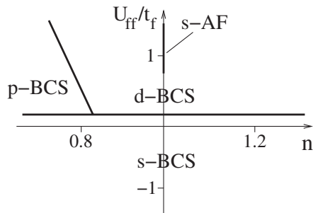
FIG. 1. Phase diagram, interaction strength, U_{ff}/t_f , vs number of fermions per site, n , for a Fermi-Bose mixture in a square lattice in 2D ( \tilde{V}/t_f = 2 , \xi = 1 ).
