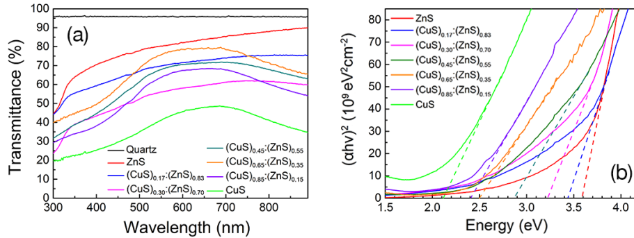
Figure 4. (a) Transmission spectra of (CuS) x :(ZnS) 1-x film (thickness~50 nm) and (b) Tauc plot of (CuS) x :(ZnS) 1-x at different Cu concentrations, from x=0 to x=1.
