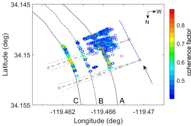
Fig. 9. Coherence peaks from 56 pings of data (colored circles) for Line 1 (see [5, Fig. 3(b)]). The broadside beam directions ( - \circ - ) and 3-dB beamwidths ( - - - ) are shown at 2-min intervals. The gray circles on the broadside beam indicate ranges at 200, 400, 600, and 800 m. The ship track is shown in blue.
