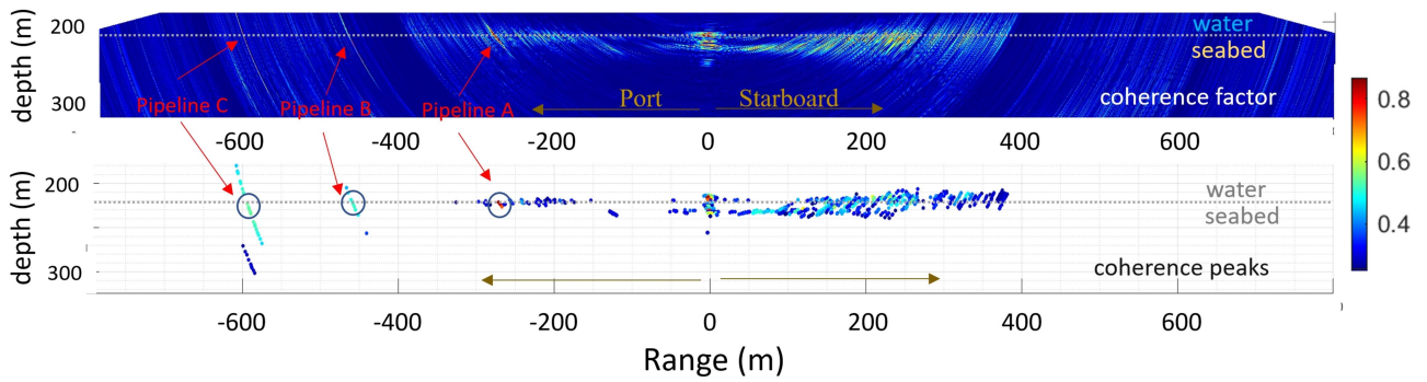
Fig. 6. Cross-track imaging for the same ping as Fig. 4(b) and (c) with added annotations for pipeline detections.
