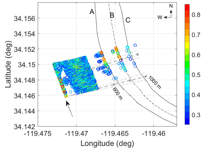
Fig. 10. Coherence peaks from 56 pings of data (colored circles) for Line 4 [see Fig. 3(b)]. The broadside beam directions ( - \circ - ) and beamwidths ( - - - ) are shown at 2-min intervals. The gray circles on the broadside beam indicate ranges at 200, 400, 600, 800, and 1000 m.
