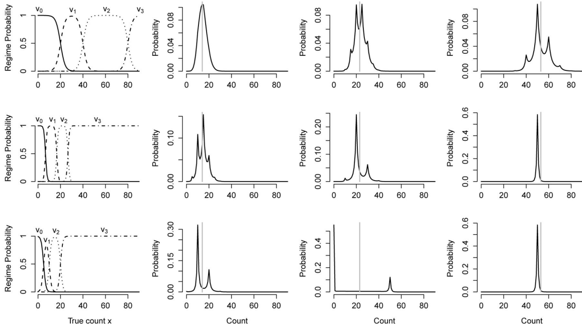
Fig 5. Heaping regimes. Each row shows a different heaping regime model with reporting probabilities for \theta_{disp} = 0.5 and \theta_{heap} = 1.5 . A gray line denotes the true counts x = 14, 23, 53 . In the first row, the regime intensities are shown with regime parameters \gamma = (0.5, -10, -20, -40) . For x = 14 , the reporting distribution is dominated by regime 0, which specifies no heaping. For x = 23 , the reporting distribution is dominated by regime 1, so rounding to nearby multiples of 5 is evident. At x = 53 , regime 2 is dominant, and the reporting distribution is peaked at multiples of 10. In the second row, \gamma = (1.5, -10, -25, -40) , and the reporting distribution for x = 53 is dominated by regime 3, so the model exhibits heaping to multiples of 50. In the third row, \gamma = (1, -5, -10, -20) .
