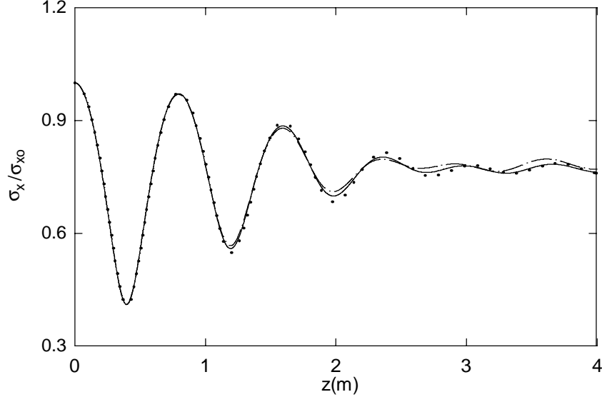
Figure 3.22: Comparison of results for the evolution of the rms beam size of the initially gaussian beam with \alpha = 5 obtained using \Delta = 12 ( -\cdot-\cdot- ), \Delta = 10 ( --- ) and \Delta = 8 ( \cdot\cdot\cdot ).
